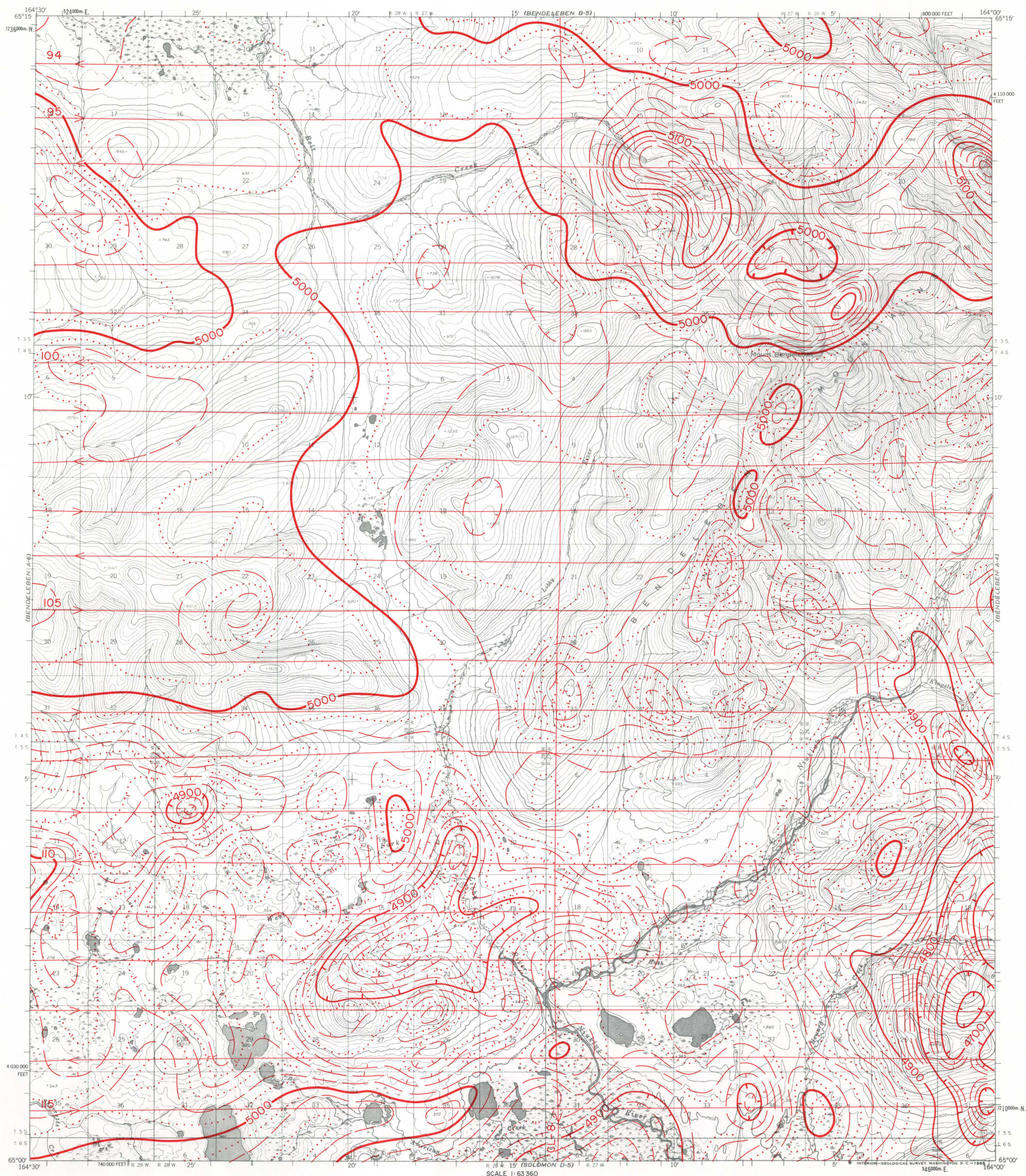
BENDELEBEN (A-5), ALASKA AEROMAGNETIC SERIES
