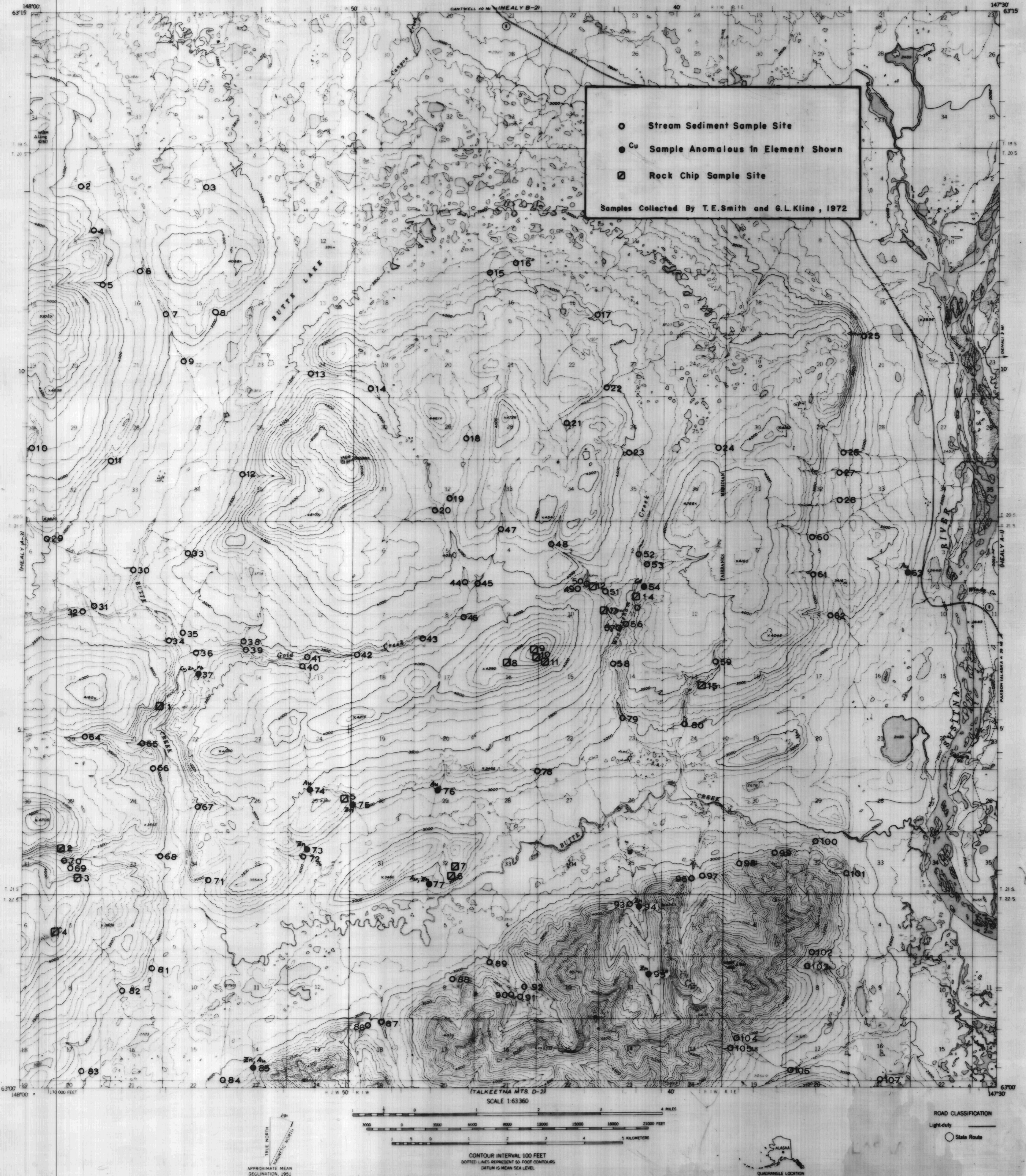
GEOCHEMICAL SAMPLE LOCATIONS, HEALY A-2 QUADRANGLE, SOUTH-CENTRAL ALASKA
