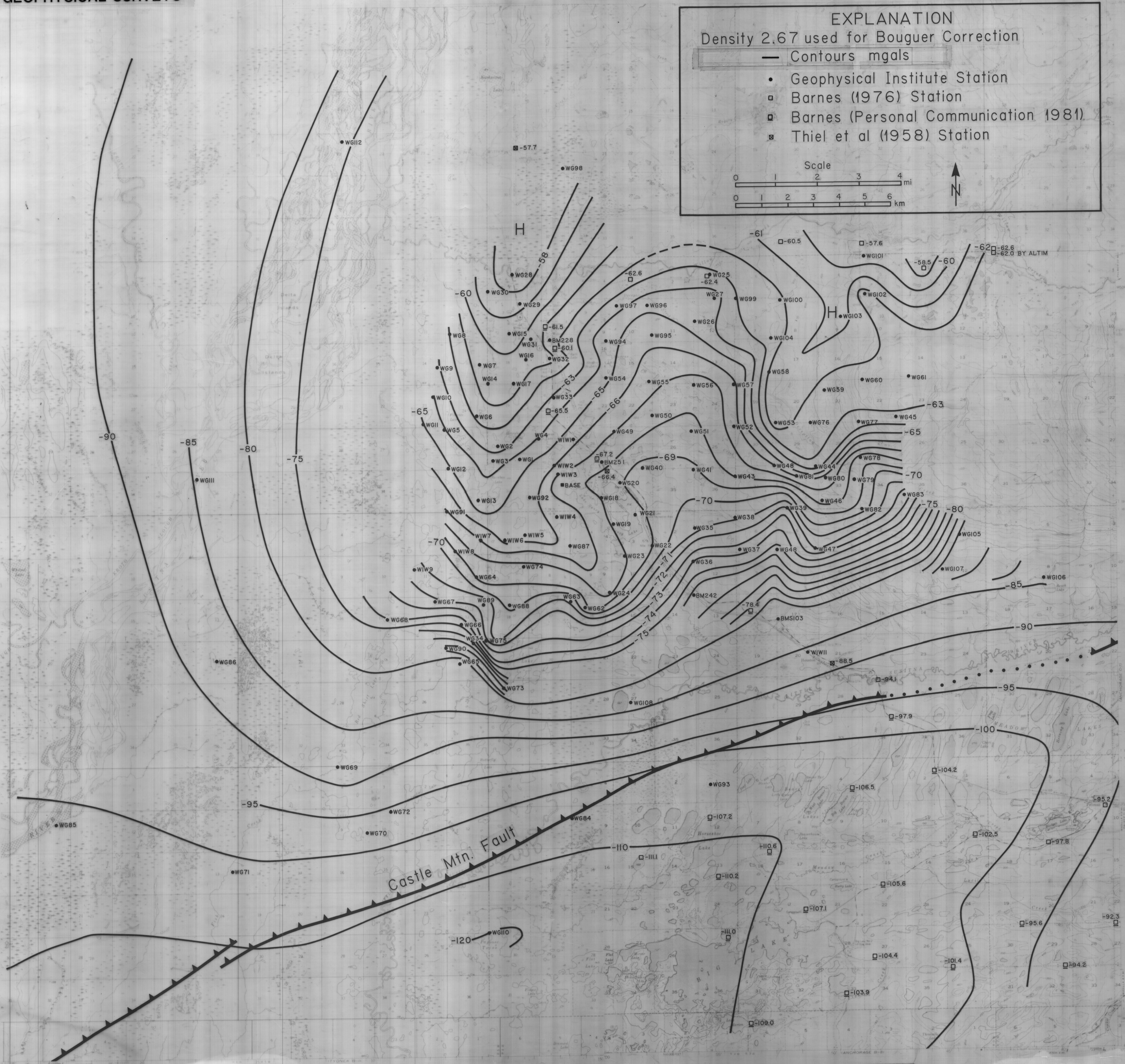
SIMPLE BOUGUER GRAVITY ANOMALY MAP OF THE LOWER SUSITNA BASIN BY EUGENE WESCOTT AND WILLIAM WITTE, 1982 GEOPHYSICAL INSTITUTE, UNIVERSITY OF ALASKA
