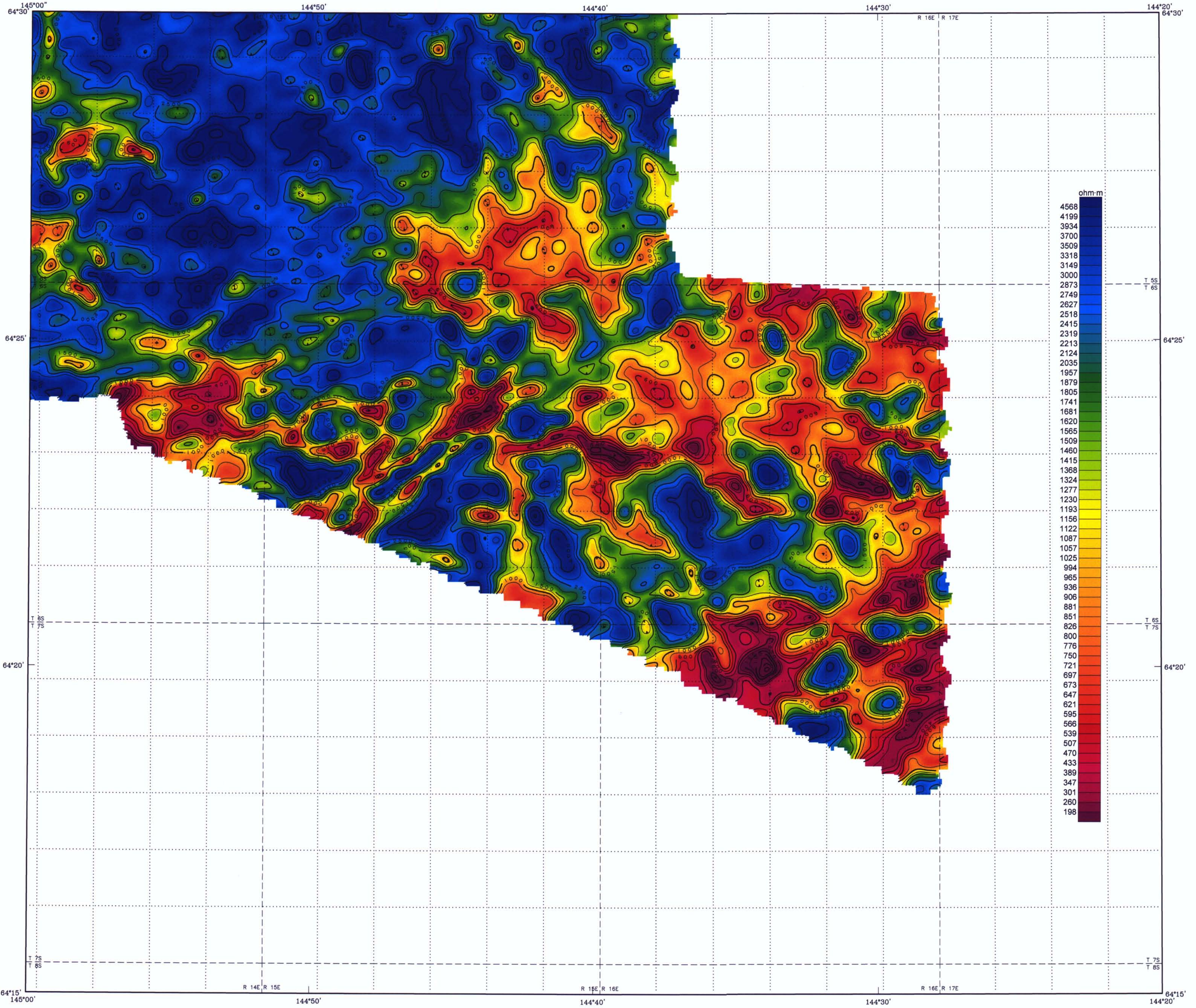
Section outlines from U.S. Geological Survey Big Delta B-1, 1973; Big Delta B-2, 1975; Quadrangles, Alaska.
