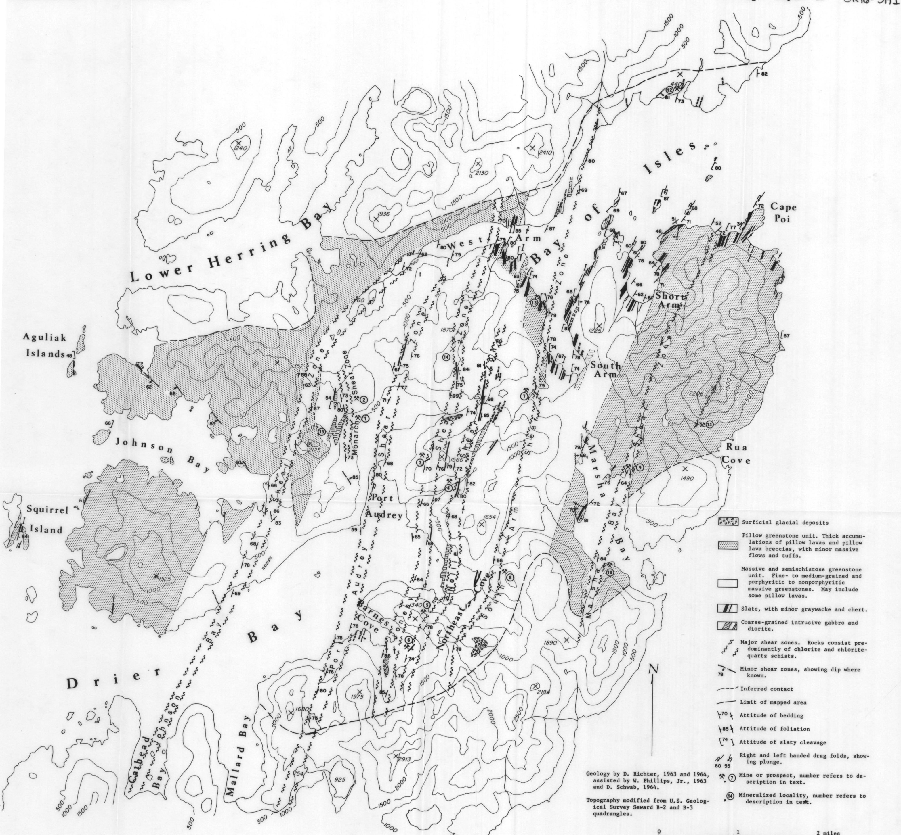
Geologic map of central Knight Island, Alaska
