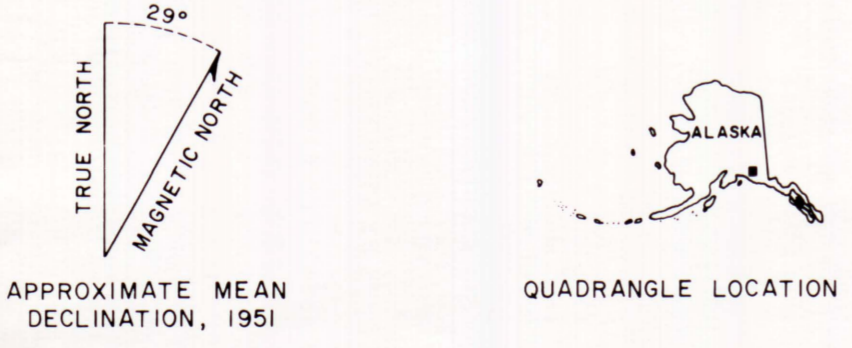
Geological - Geochemical Map of Area Around the Spirit Mountain Nickel - Copper Prospect
