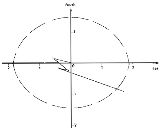
Figure 22. Apparent strain path of survey station 17.
