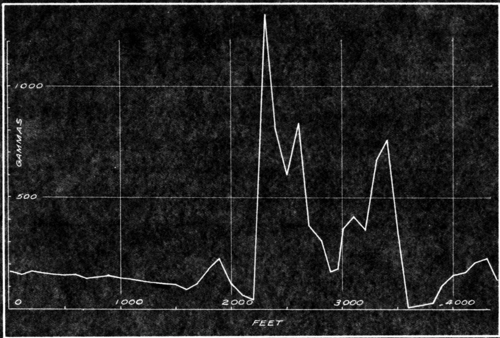
Fig. 6. - Magnetic profile along Line 4.
