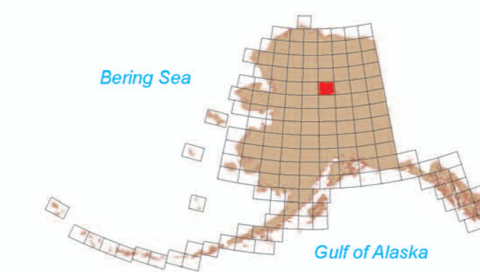
Location map for Bettles Quadrangle
