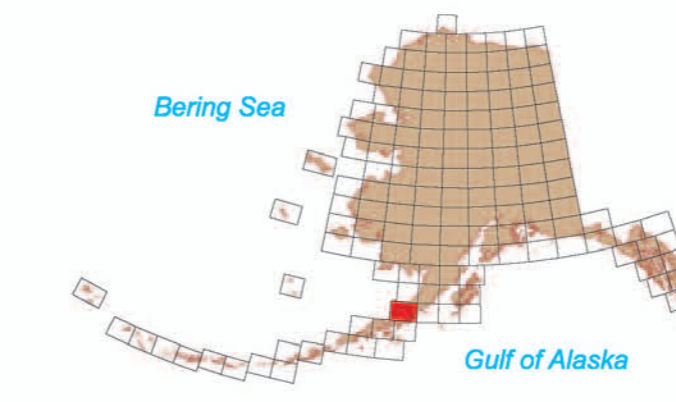
Location map for Chignik Quadrangle
