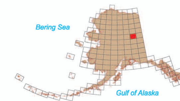
Location map for Circle Quadrangle
