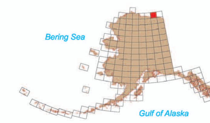
Location map for Flaxman Island Quadrangle
