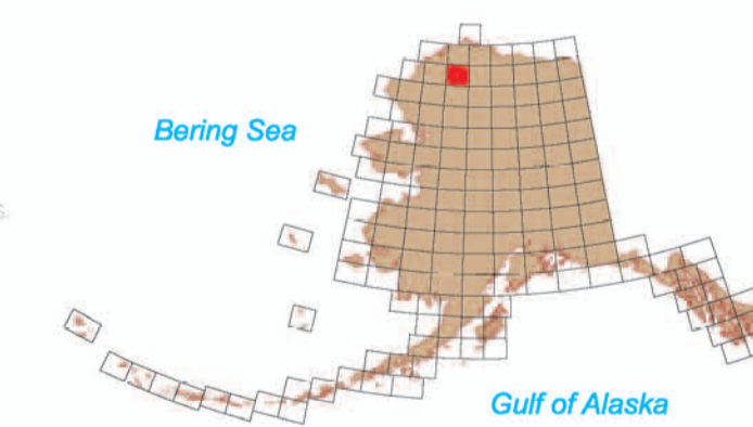
Location map for Lookout Ridge Quadrangle
