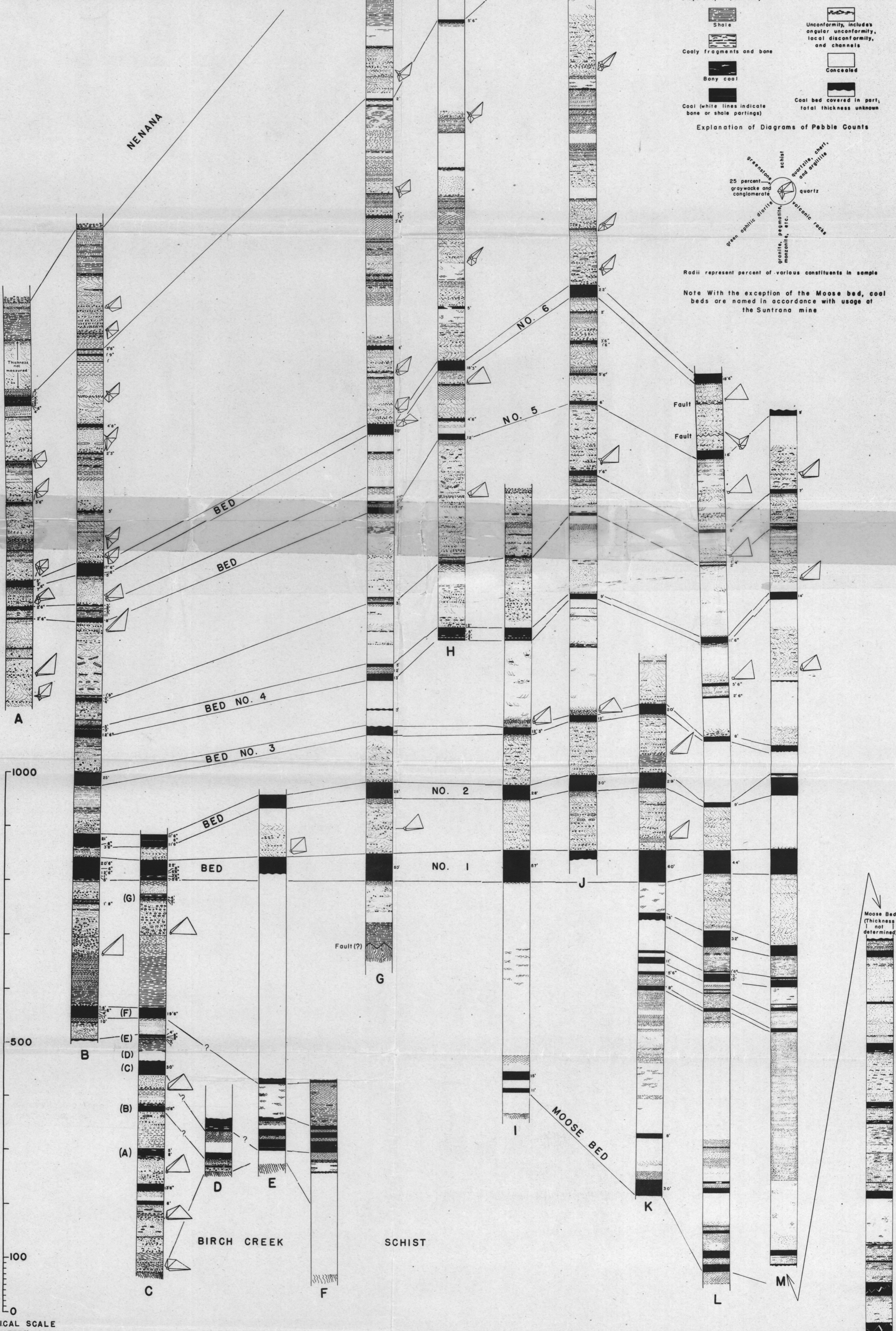
FIG. 4: STRATIGRAPHIC SECTIONS SHOWING CORRELATIONS OF COAL BEDS IN THE VALLEY OF THE HEALY RIVER, ALASKA
