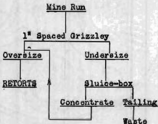
Flow-sheet of ore treatment.
