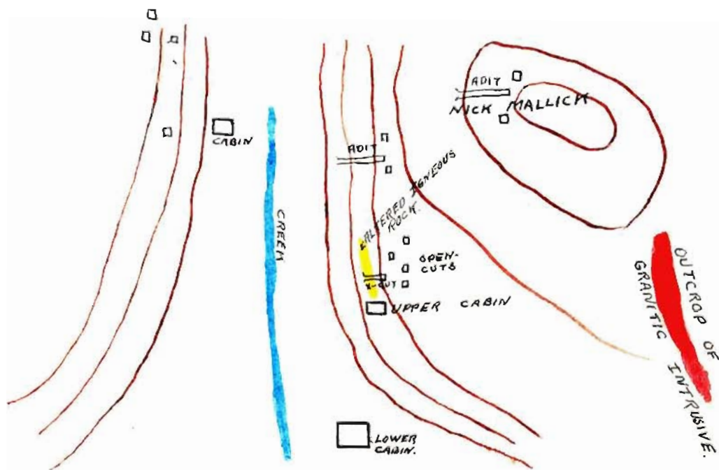
Sketch showing plan of Fuller and Willis prospect.
