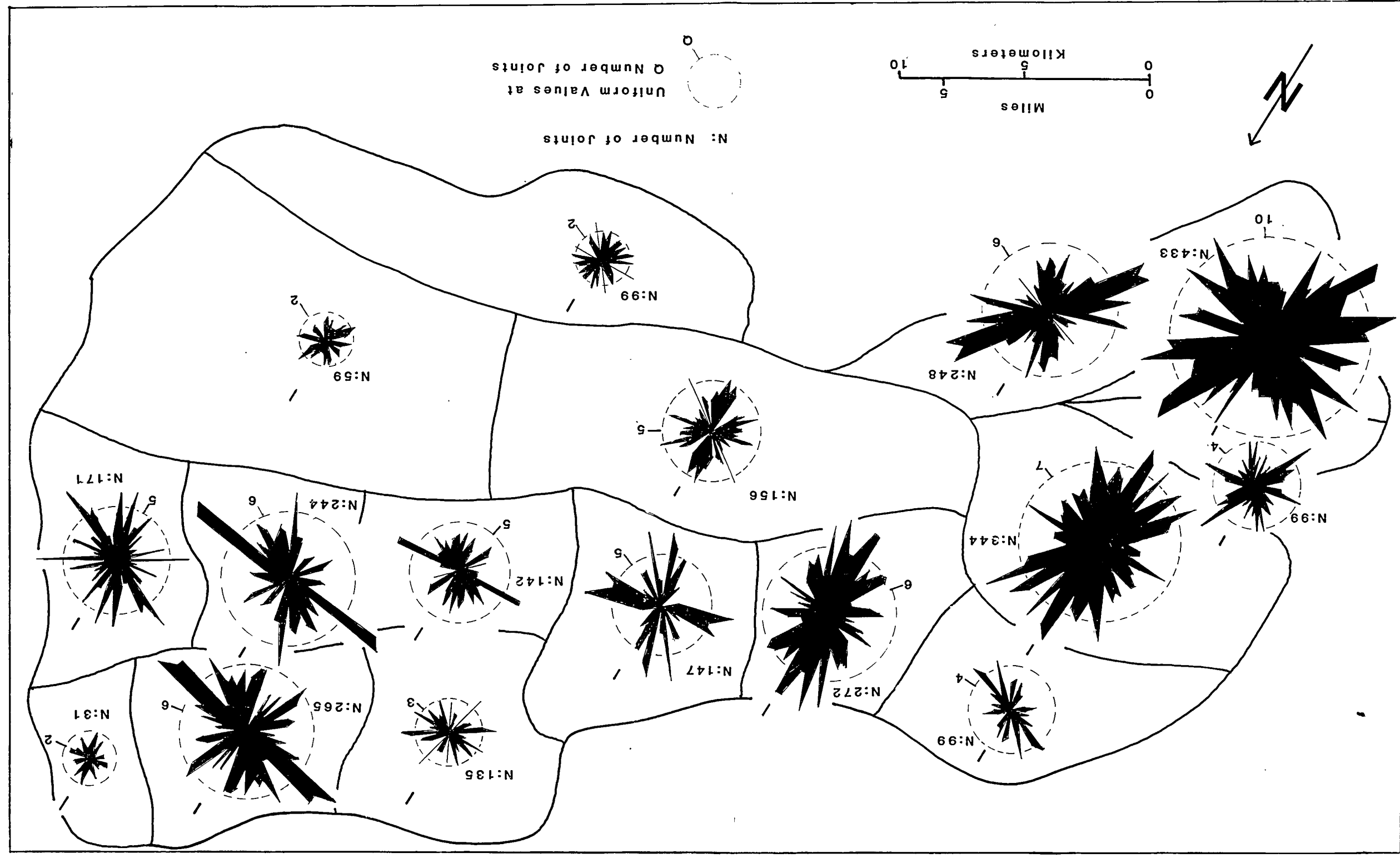
Plate 1l Rose diagram plots, Joints
