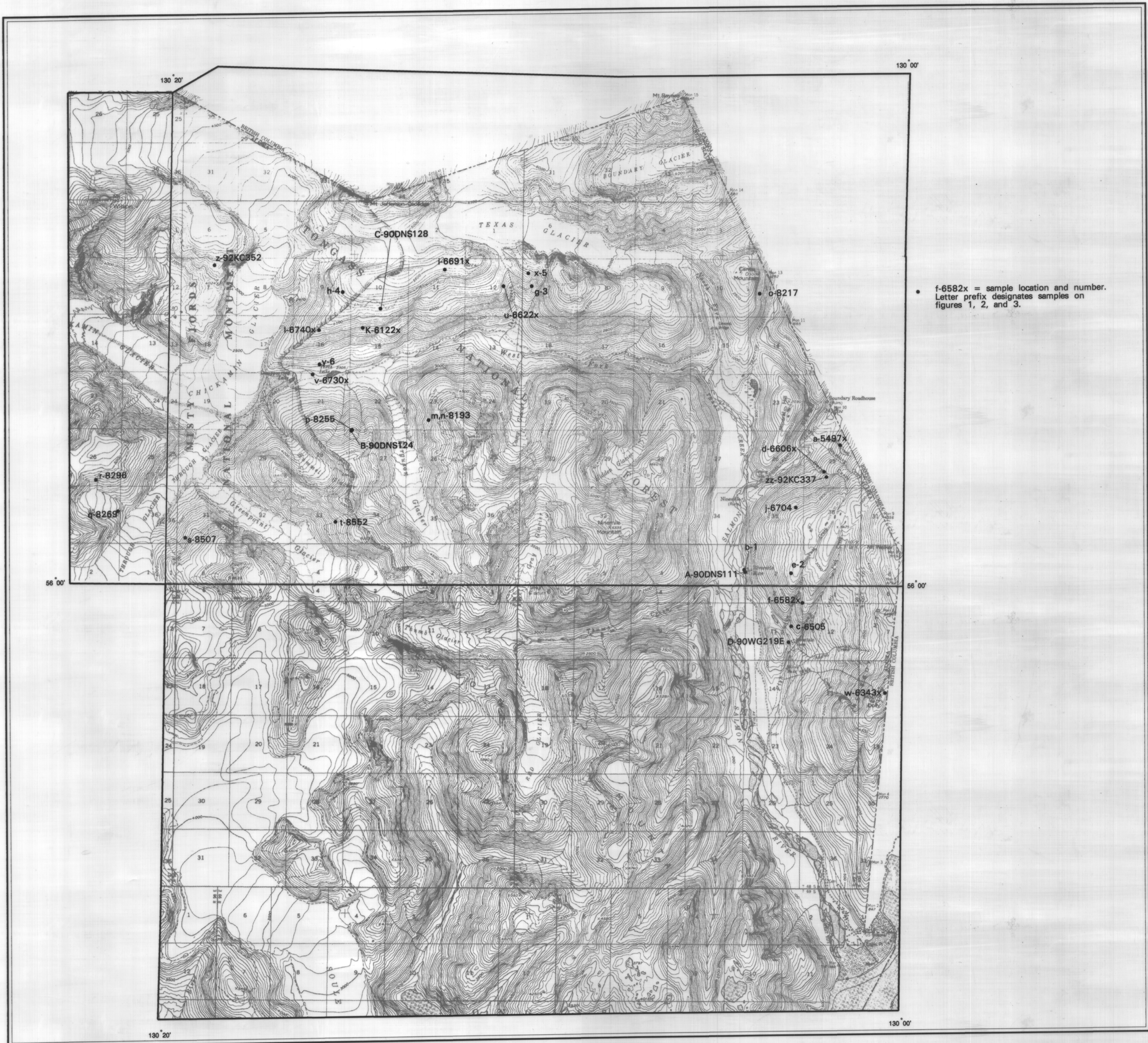
Plate 1. Locations of Galena Lead Isotope Samples, Hyder Area, Alaska (portions of Ketchikan D-1, Bradfield Canal A-1 and A-2 Quadrangles)
