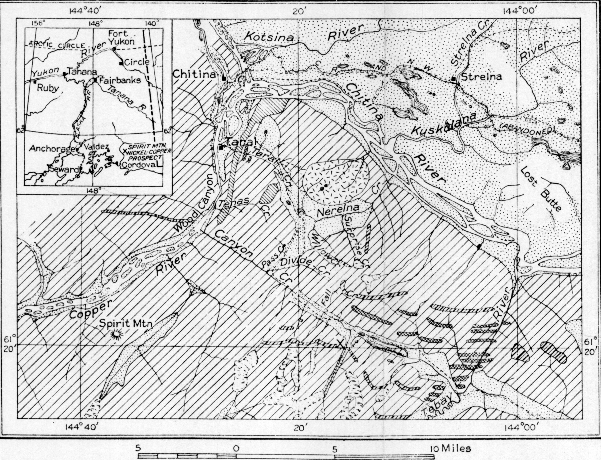
FIGURE 3.—Map of part of the Copper River region, Alaska, showing location and geologic setting of the Spirit Mountain nickel-copper prospect.
