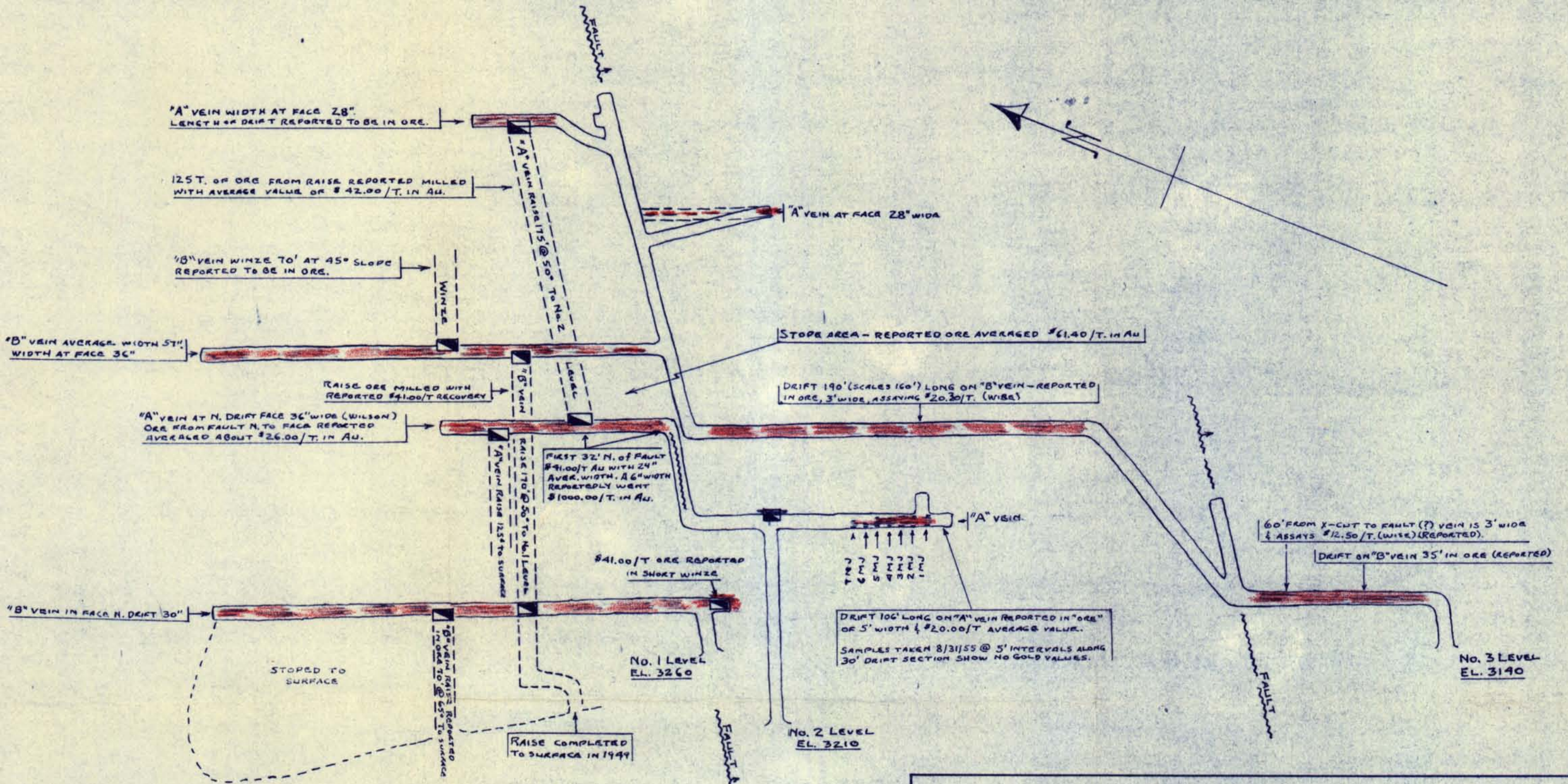
MINE PLAN SHOWING EXTENT OF MINE WORKINGS ON THE SKEEN & LECHNER GOLD PROPERTY FROM ORIGINAL DISCOVERY IN 1907 TO DATE PROPERTY HELD SINCE 1939 BY FALLS CREEK MINING COMPANY, SEATTLE LOCATED ON FALLS CREEK, MOOSE PASS DISTRICT, SEWARD PRECINCT SEWARD QUARRANGLE TRACED FROM COPY OF COMPANY MAP by MW Jaeger , MINING ENGINEER TERR. DEPT. OF MINES ANCHORAGE, ALASKA JANUARY 30, 1956 Scale 40' 20' 0' 40' 80' MAP I
