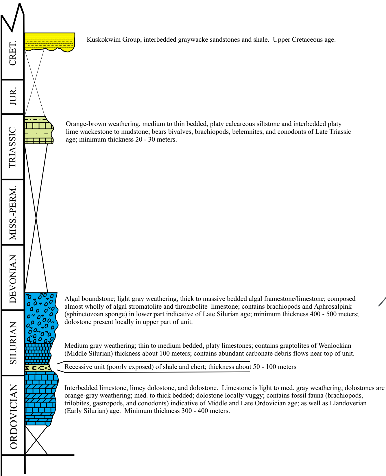
Figure 4. Generalized stratigraphic column for the south side of the Sleetmute anticlinorium.
