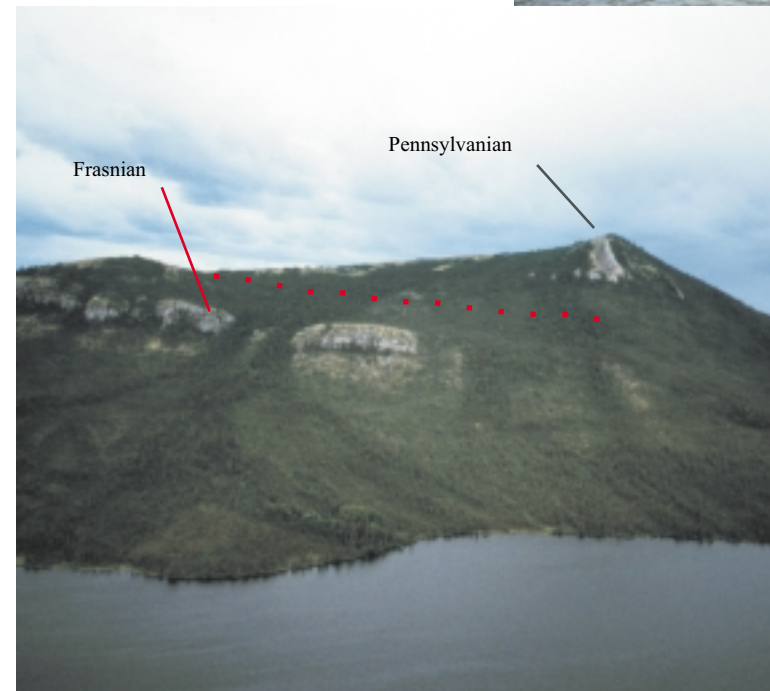
Pennsylvanian shelf carbonates in fault contact above Frasnian age shelf carbonates.
