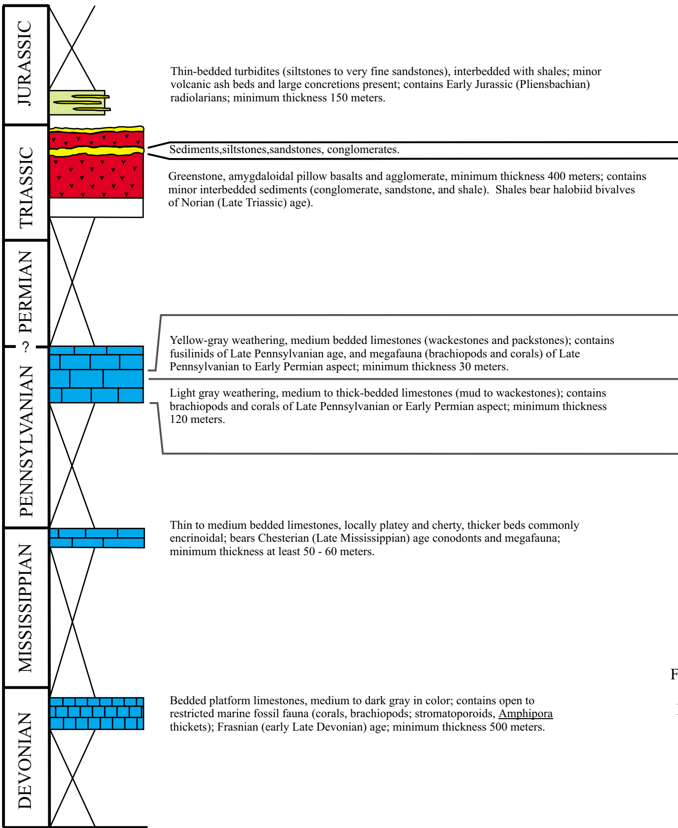
Figure 6. Generalized stratigraphic column of the Lime Lakes-Gagaryah River area.
