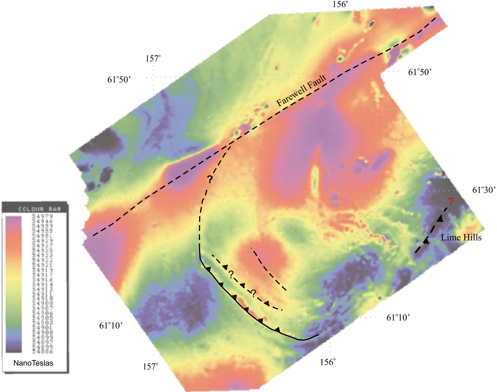
Figure 7. Aeromagnetic survey results for the Holitna region. Note the aeromagnetic high north of 61°10' north latitude and centered on 156° west longitude. The origin of this high is unknown. The linear trends visible in the southern part of the survey area correspond to south- and southwest-vergent fold and thrust structures shown in the DSL Dab units on Figure 2. Faults are dashed where concealed or inferred, and barbs are shown on upper sheet for thrust faults. The aeromagnetic survey results are available from DGGS as Public-Data File 98-29.
