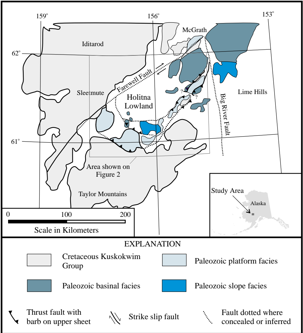
Figure 1. Map showing the location and generalized geology of the Holitna Lowland and surrounding hills discussed in this report. The study area straddles the Lime Hills, Sleetmute, and Taylor Mountains 1:250,000-scale quadrangles
