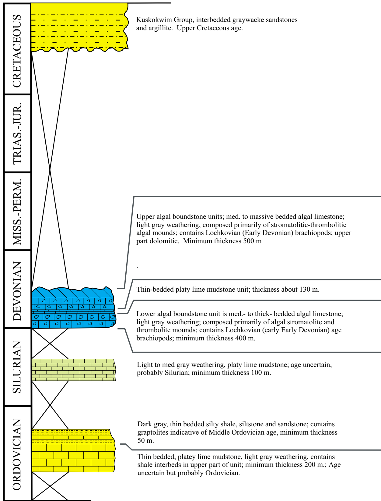
Figure 5. Generalized stratigraphic column of the Lime Hills-Why Lake area.
