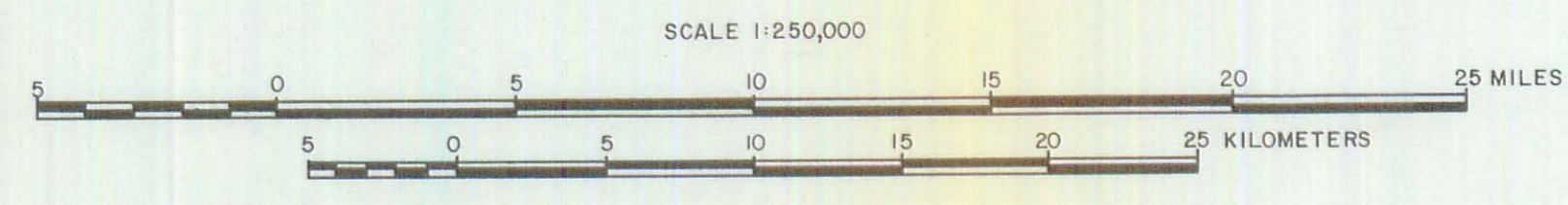
Stream sediment sample locations—U.S. Bureau of Mines—Kanuti—Hodzana Project
