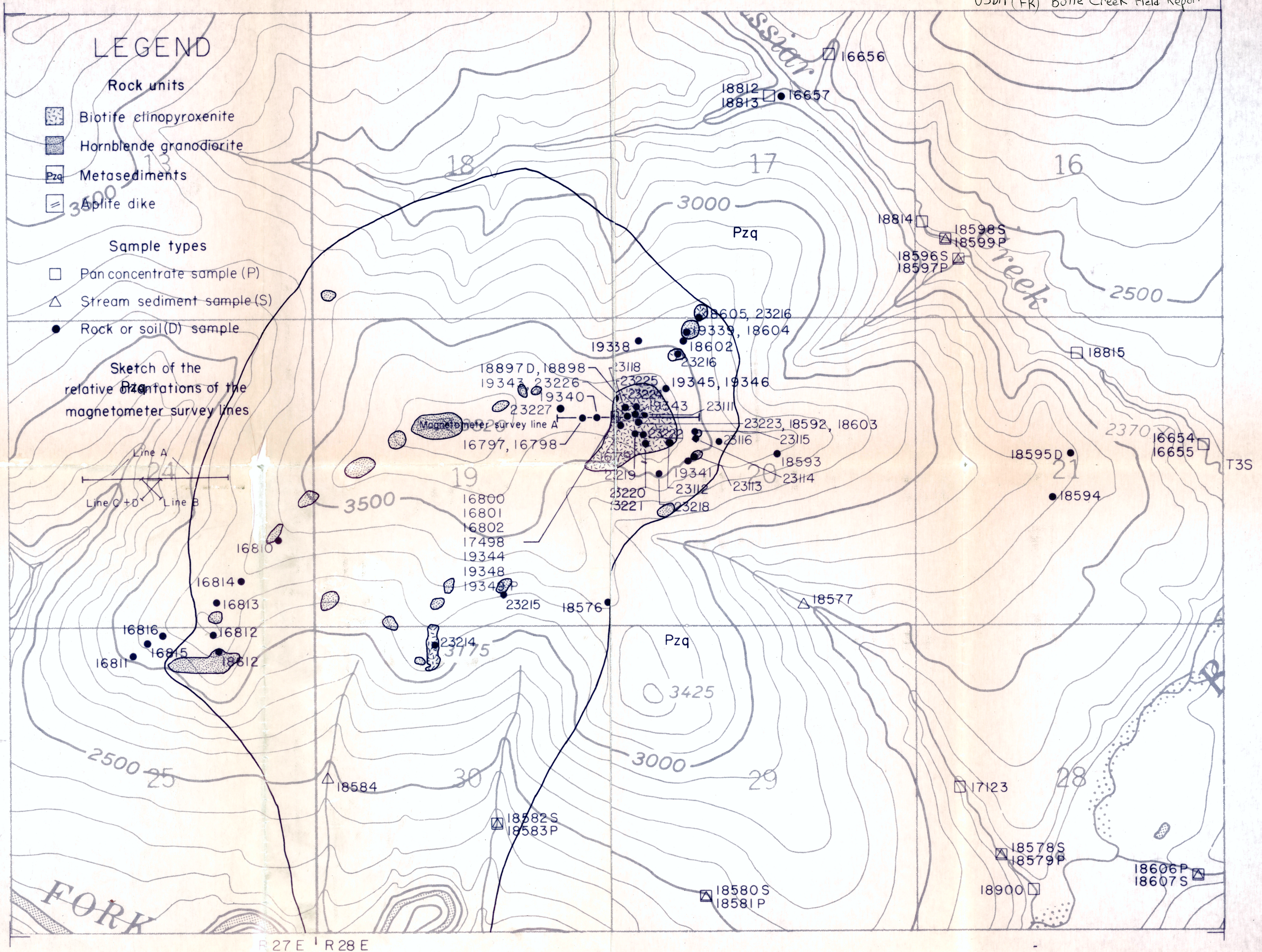
Figure 2. Geology and sample locations
