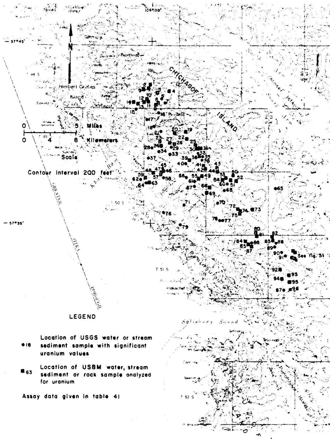
FIGURE 30. - Uranium investigations, sample locations (Base adapted from USGS 1:250,000 scale Sitka quad.)
