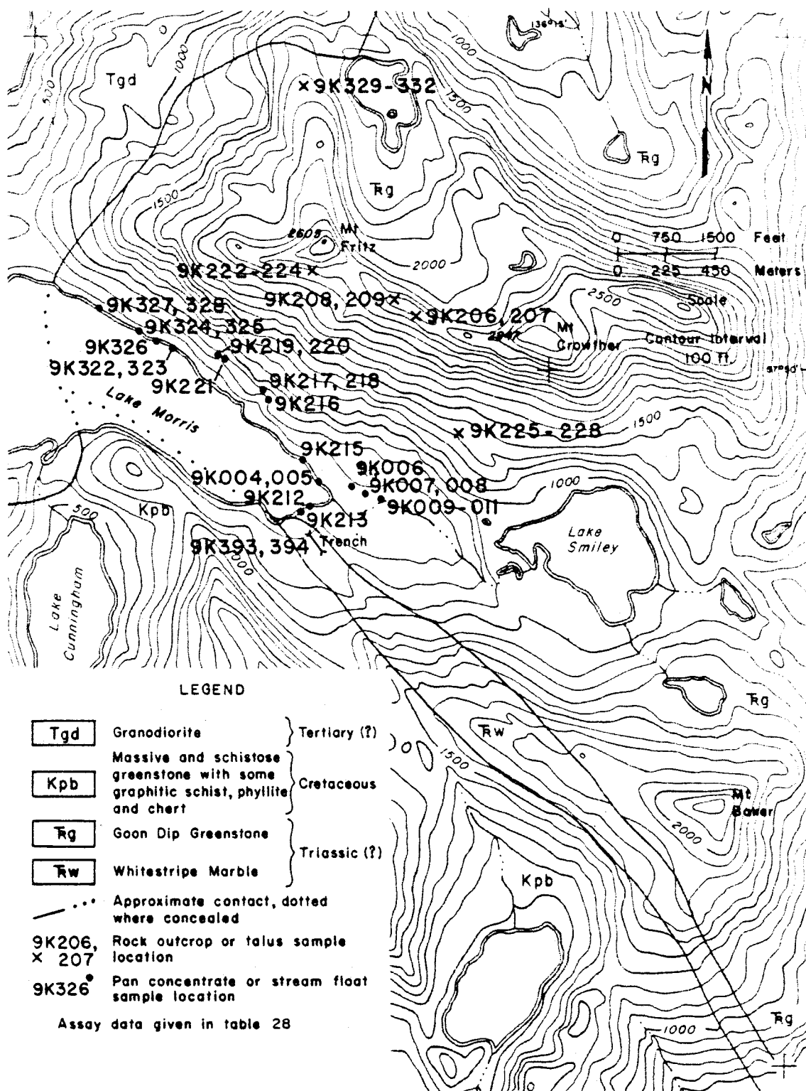
FIGURE 19. - Mt. Fritz - Mt. Crowther - Lake Morris, sample locations (Geology adapted from Johnson and Karl, 1982)
