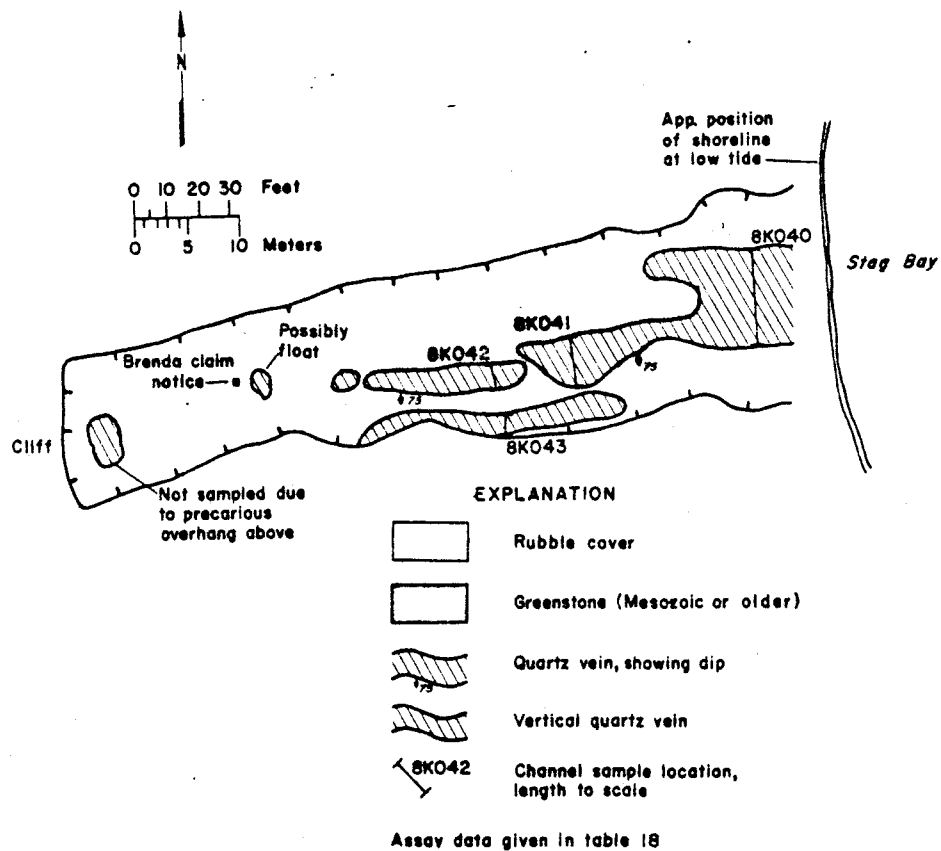
FIGURE 8. - Brenda vein, sample locations
