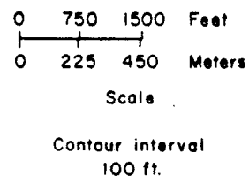
FIGURE 6. - Mine Mountain and vicinity, sample locations (Geology adapted from Johnson and Karl, 1982)
