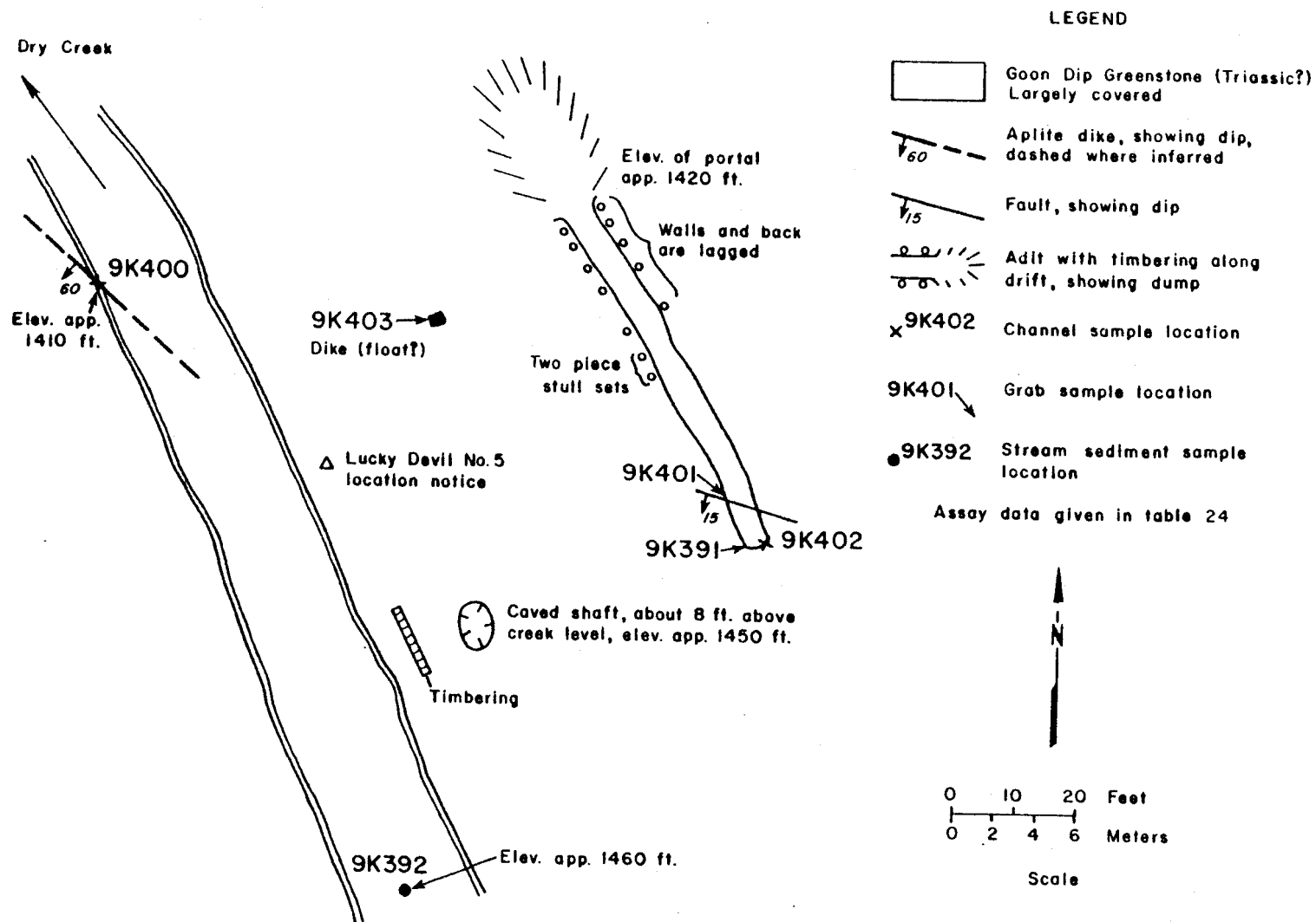
FIGURE 16. - Upper "old" adit, Mt. Baker, sample locations
