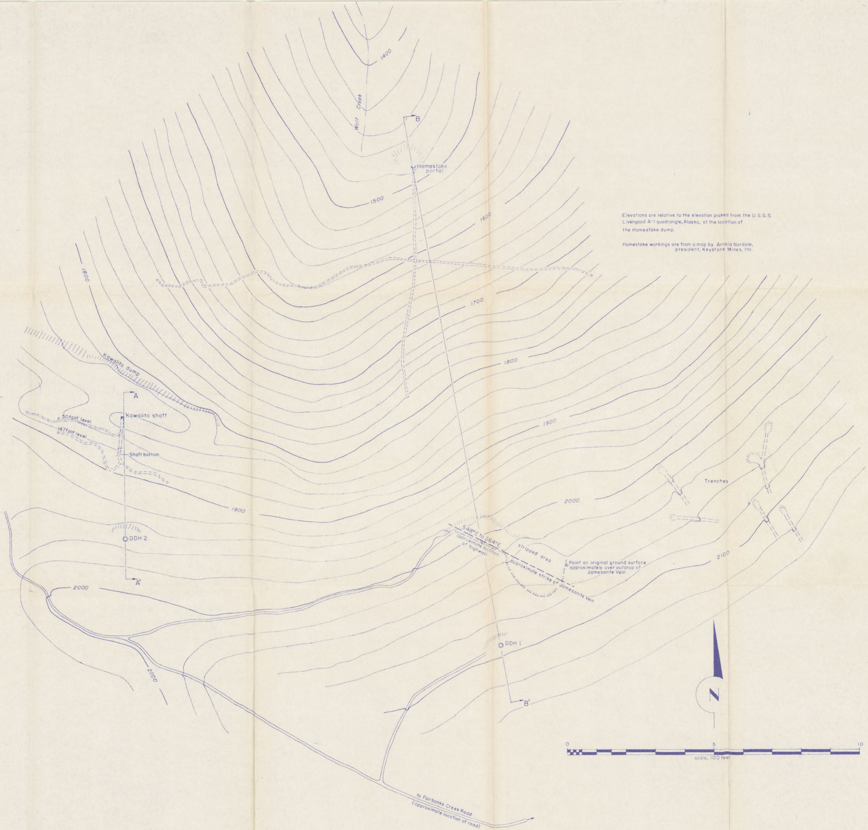
FIGURE 2.- Plan, Keystone Diamond Drill Holes Fairbanks Creek, Wolf Creek Divide Area, Fairbanks District, Alaska
