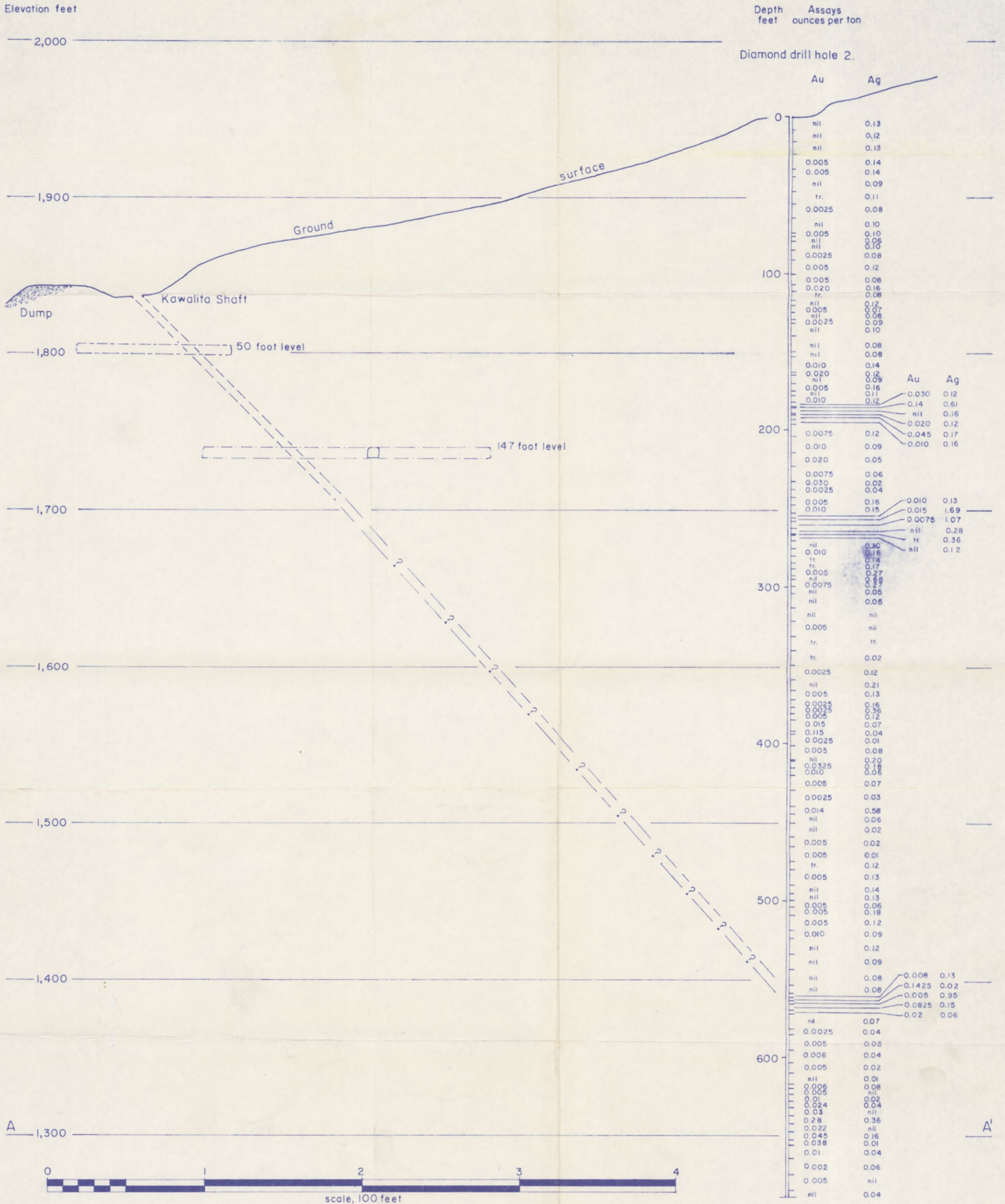
FIGURE 3.- Section A-A', through diamond drill hole 2., Keystone property Fairbanks Creek, Wolf Creek Divide Area, Fairbanks District, Alaska.
