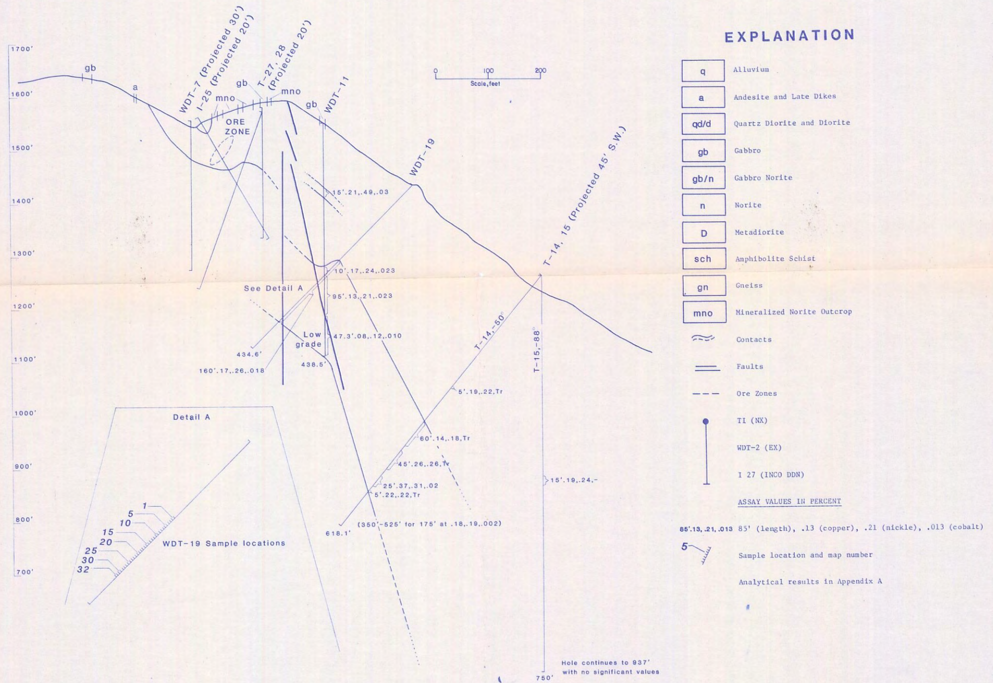
FIGURE 11. - Takanis Area, Section T-5-5, showing geology and diamond drill hole WDT-19 location. Inset shows drill hole WDT-19 sample locations. Modified from Salisbury and Dietz, Inc. map (7)
