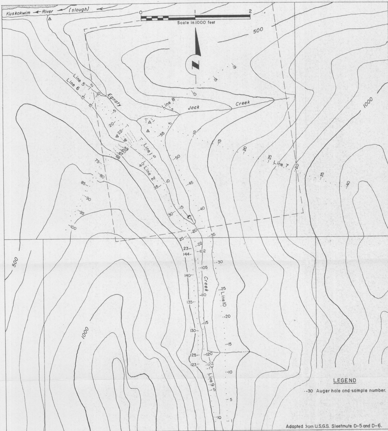
FIGURE 3.- Location map of Auger samples at Egnaty Creek Alaska.
