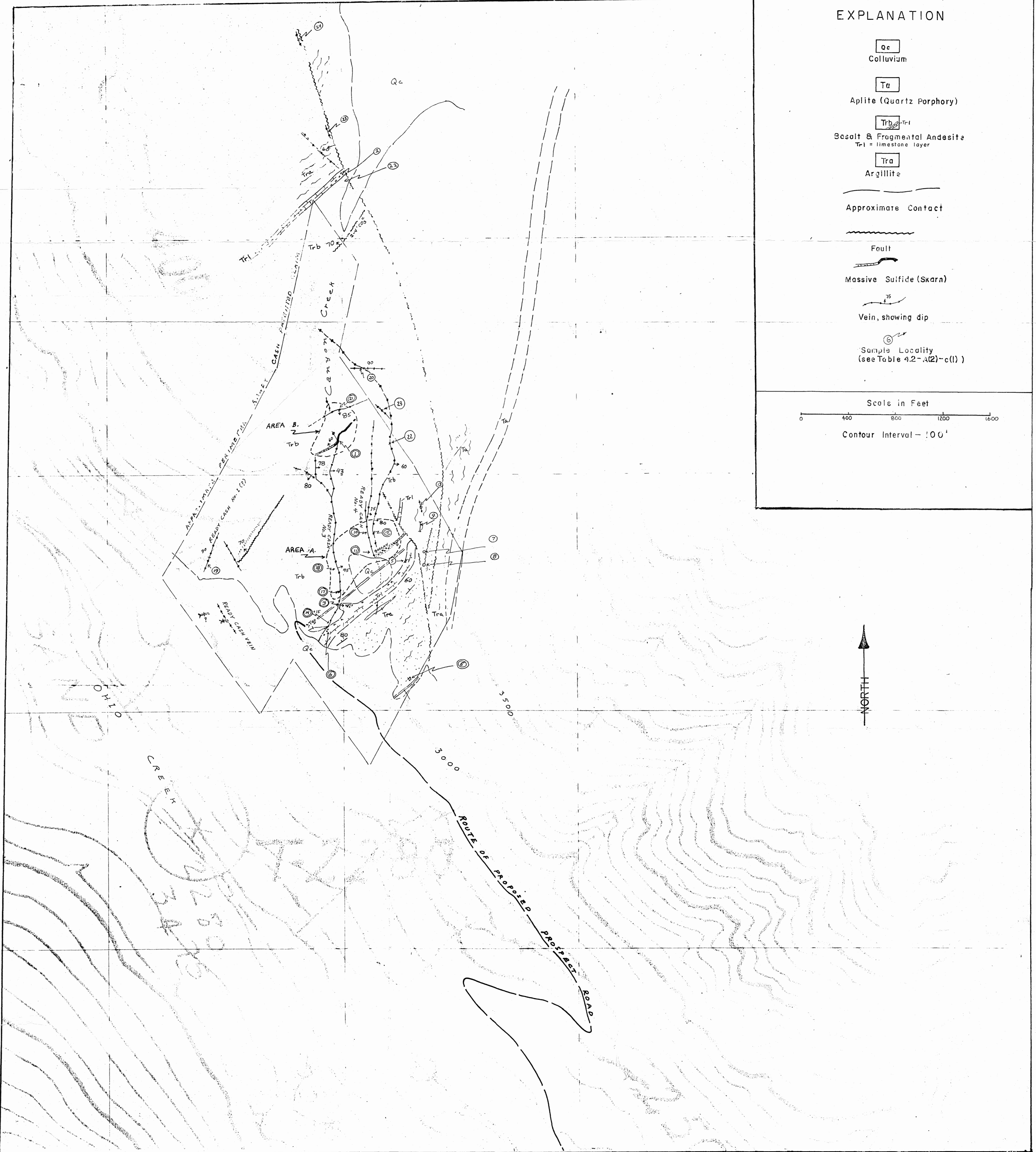
FIGURE 4.2-A(2)-C -- MAP OF READY CASH AREA, HEALY A-6 QUAD, ALASKA SHOWING SAMPLE LOCATIONS
