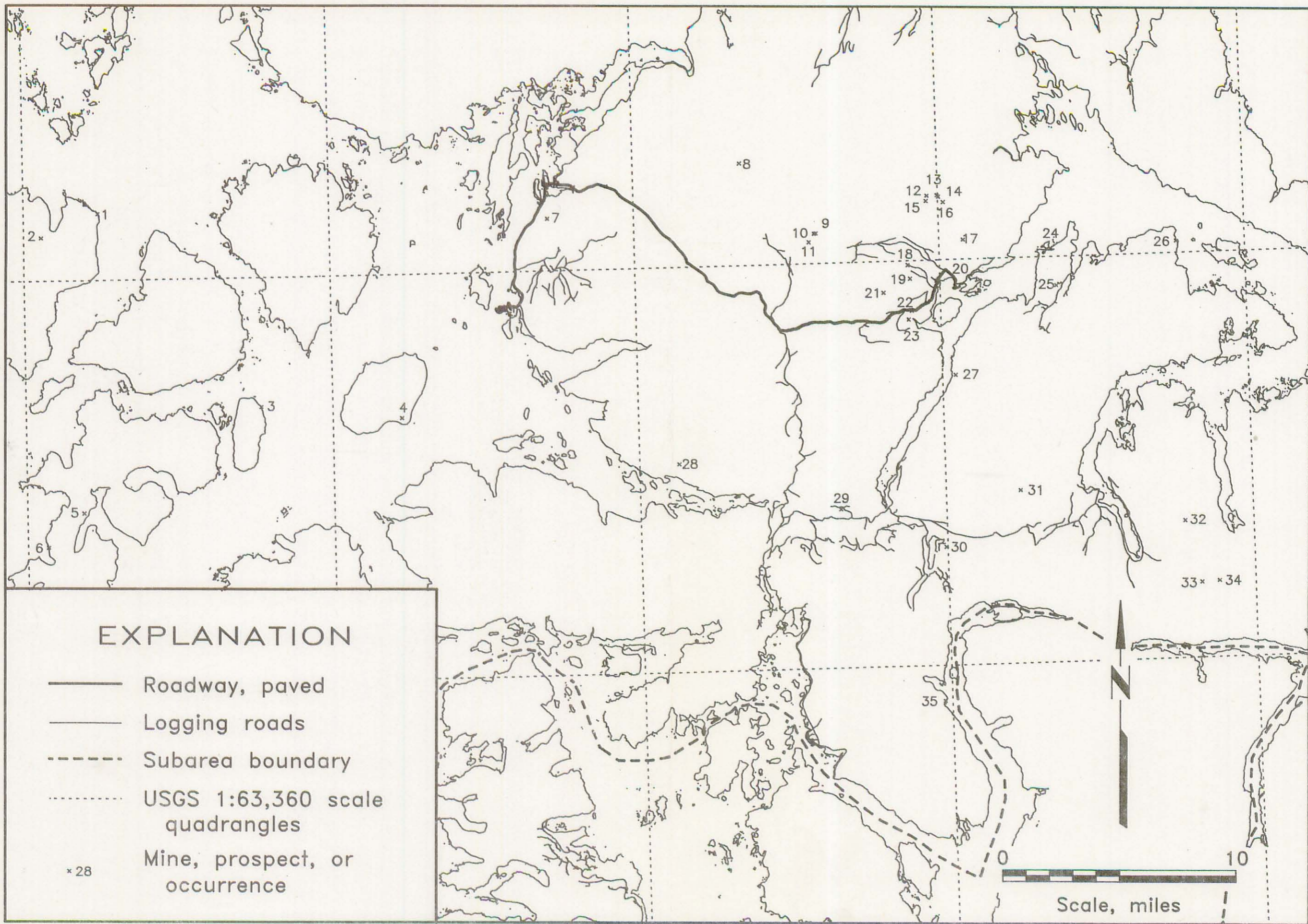
Figure 8. - Mines, prospects, and occurrences: Craig subarea.
