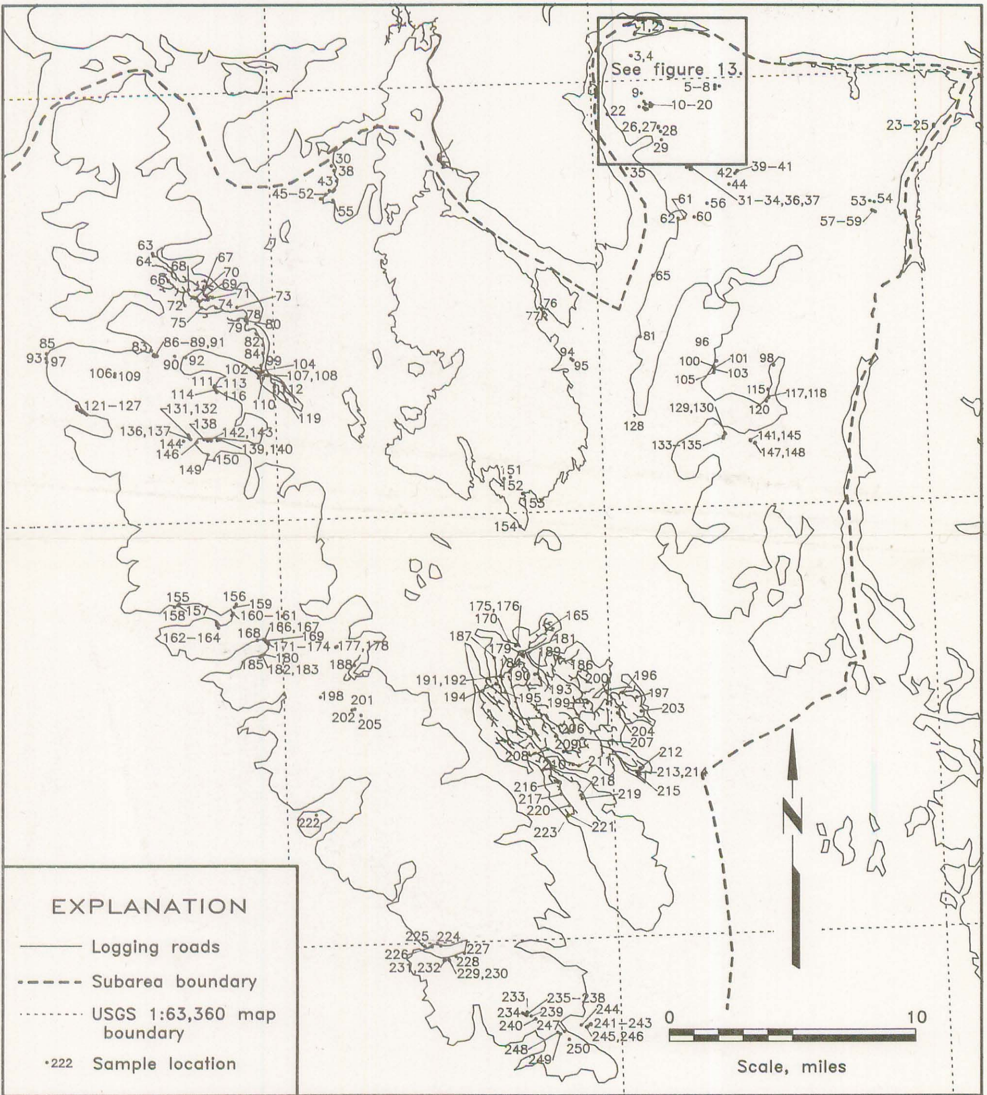
Figure 12. - Sample location map: Dall Island subarea.
