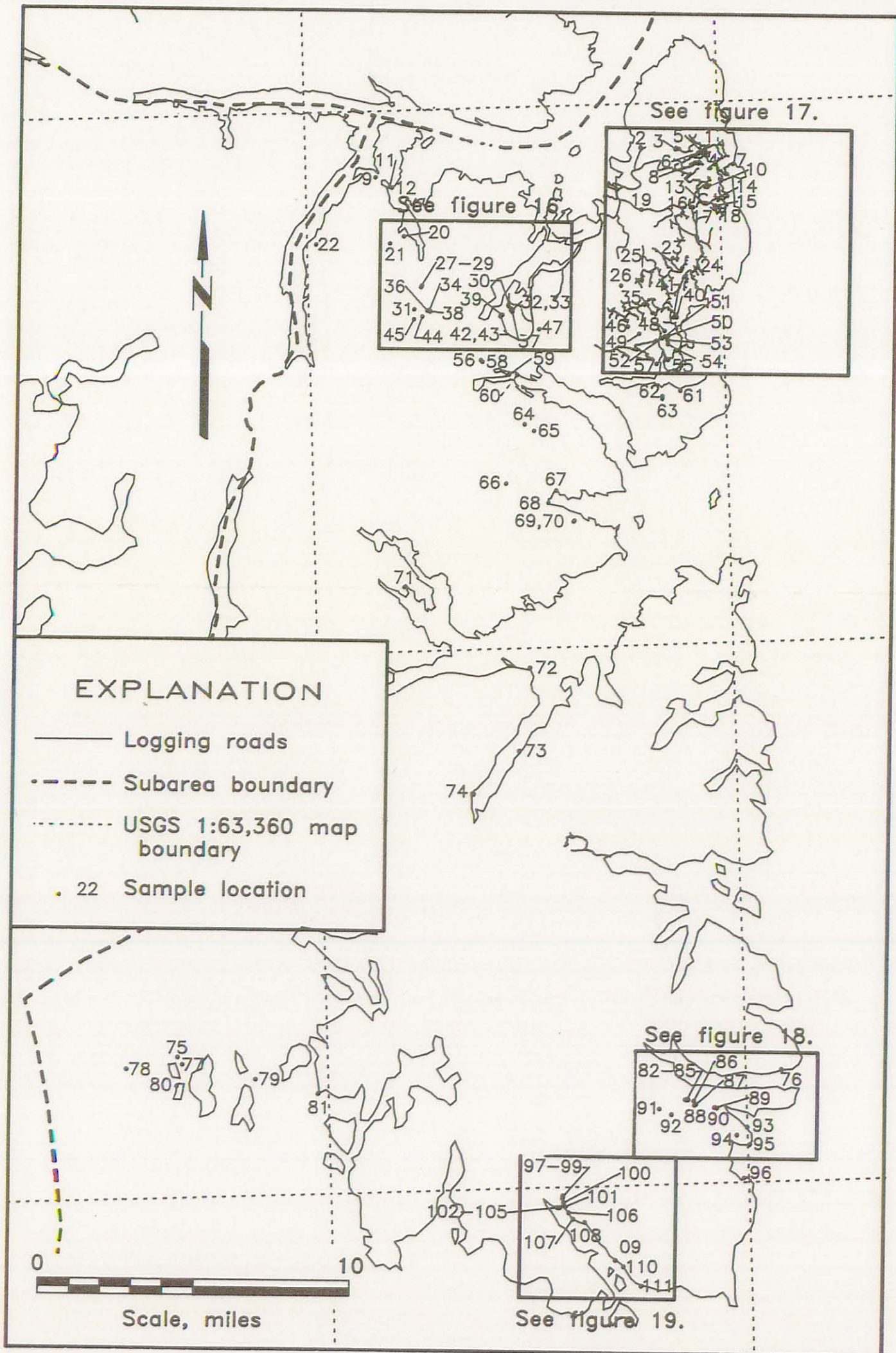
Figure 15. - Sample location map: Southeast Prince of Wales Island subarea.
