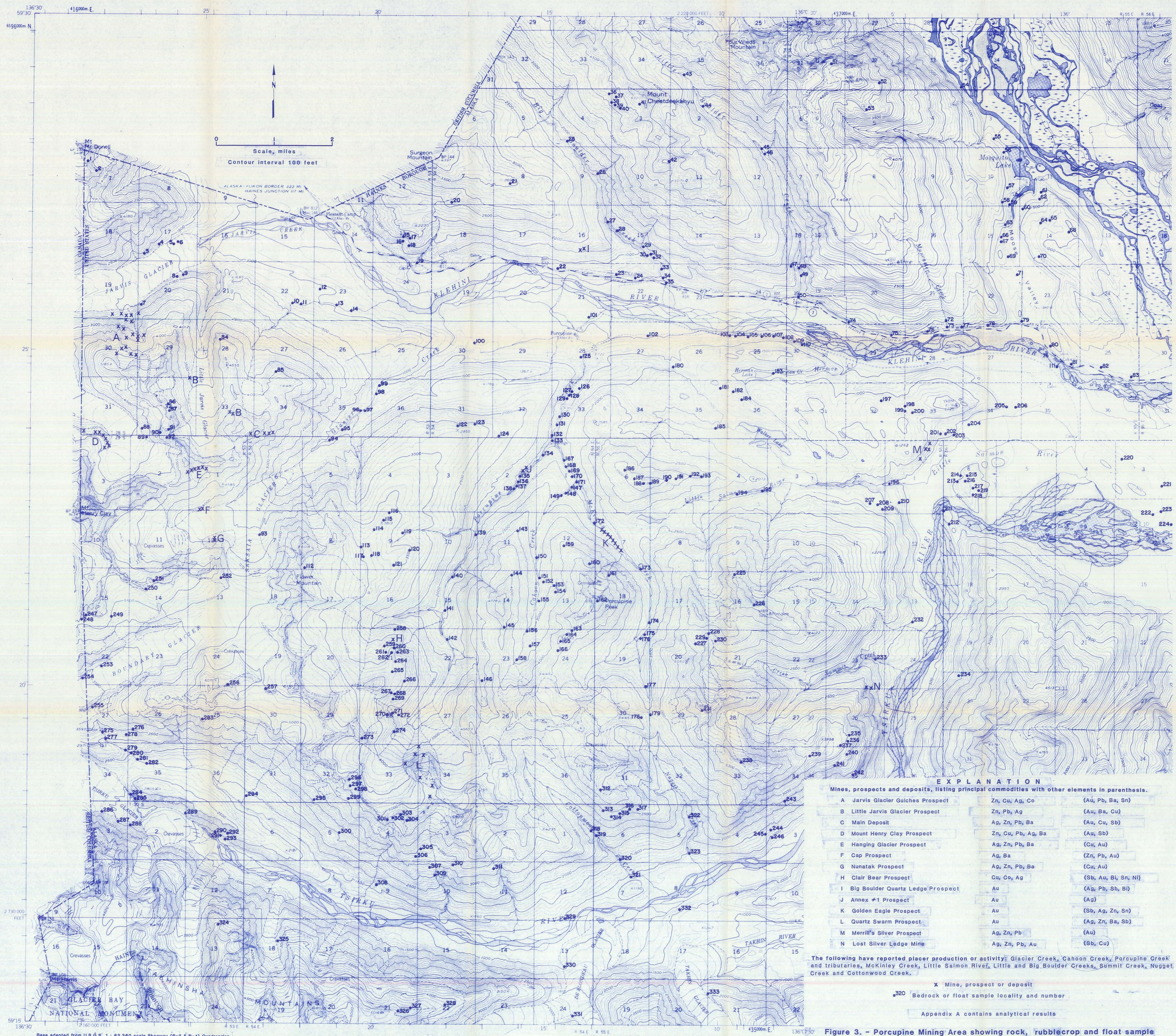
Figure 3. - Porcupine Mining Area showing rock, rubble/crop and float sample localities, and lode mines, prospects and deposits.
