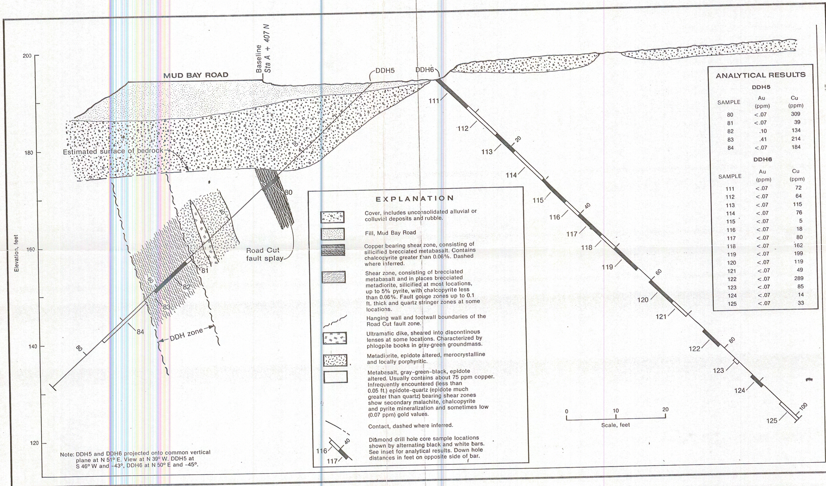
Figure 10.— Road Cut prospect vertical cross-section XS1 showing DDH5 and DDH6.
