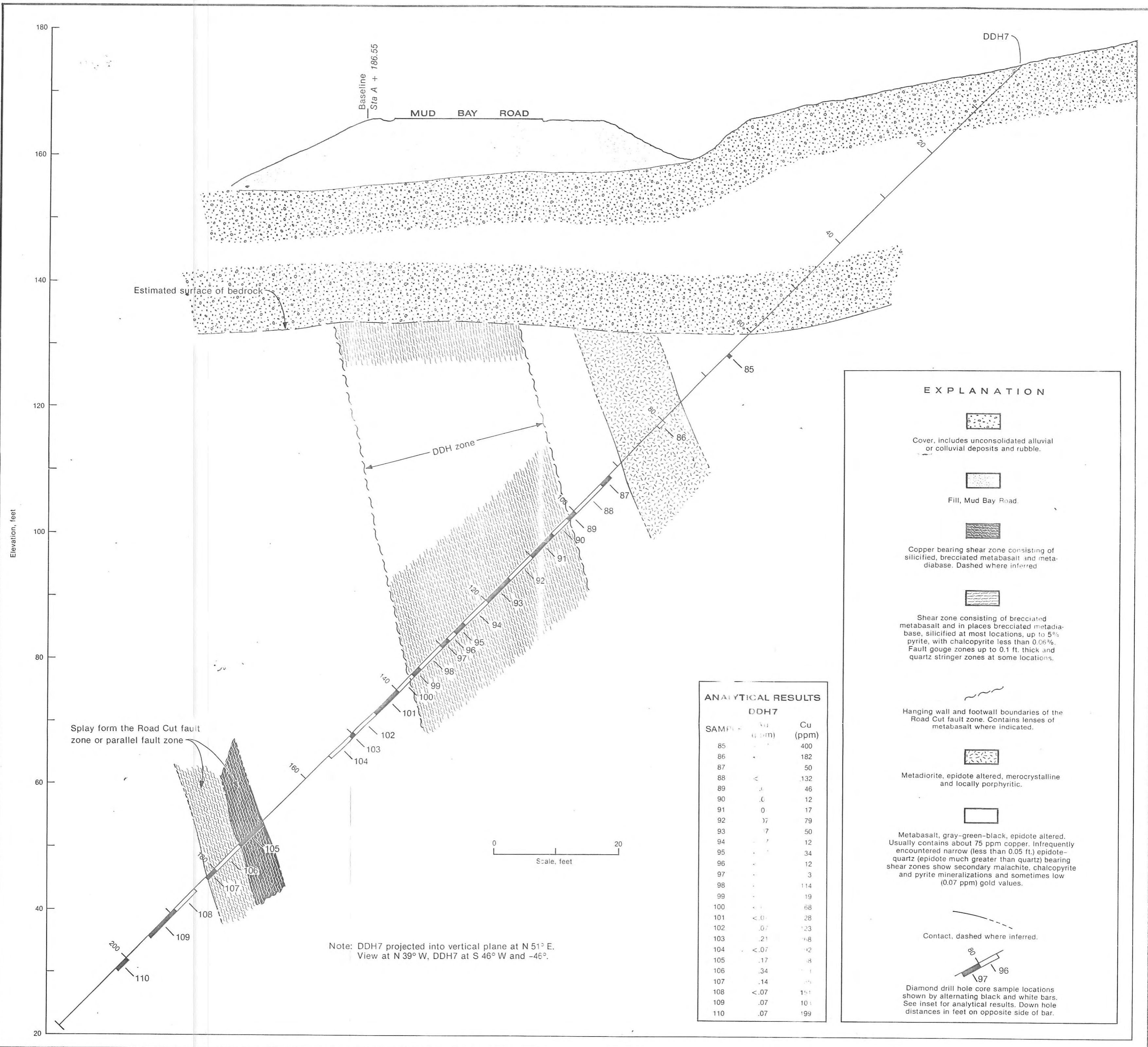
Figure 14.— Road Cut prospect, vertical cross-section XS5, showing DDH7.
