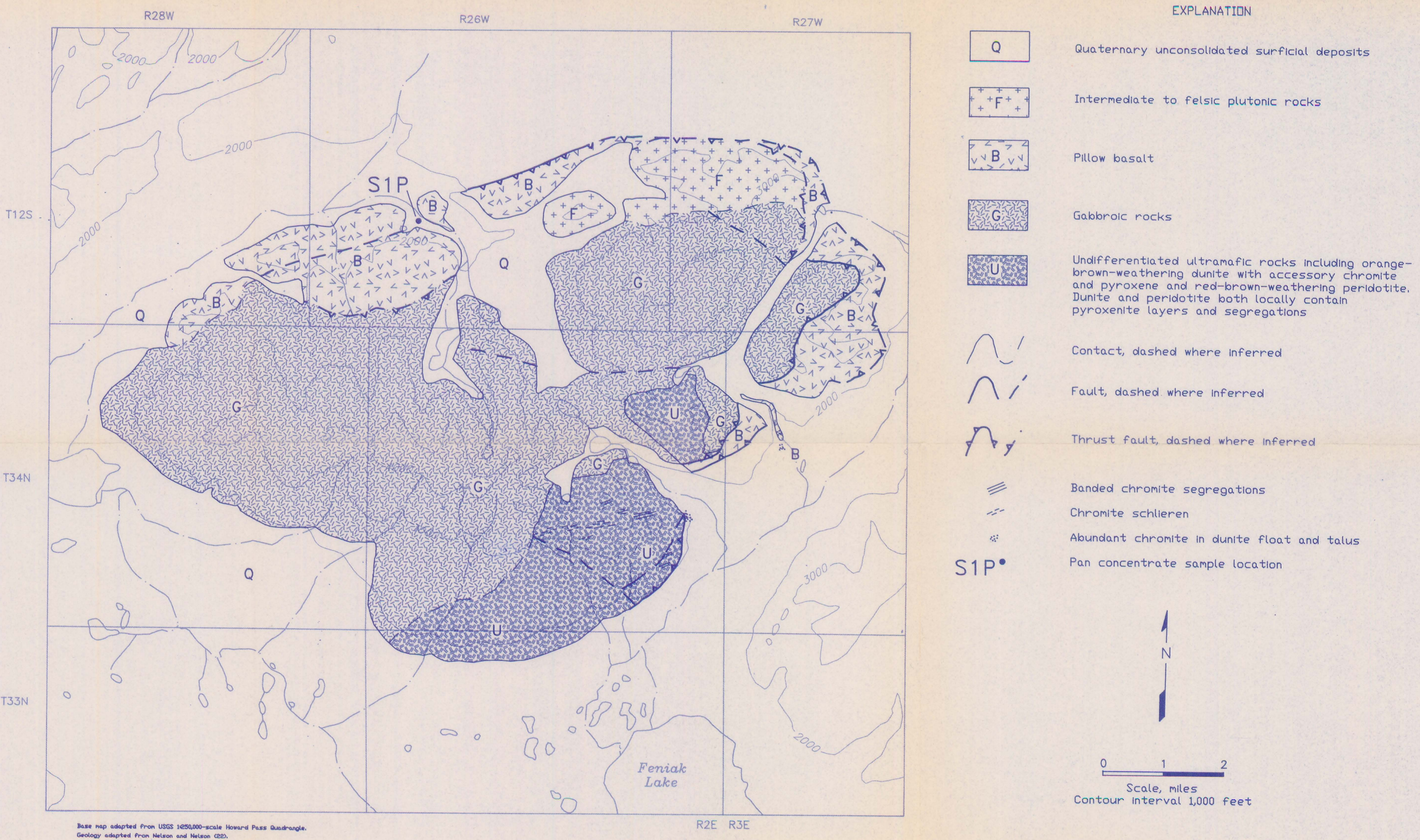
Figure 24. - Geologic map of Siniktanneyak Mountain, showing chromite occurrences.
