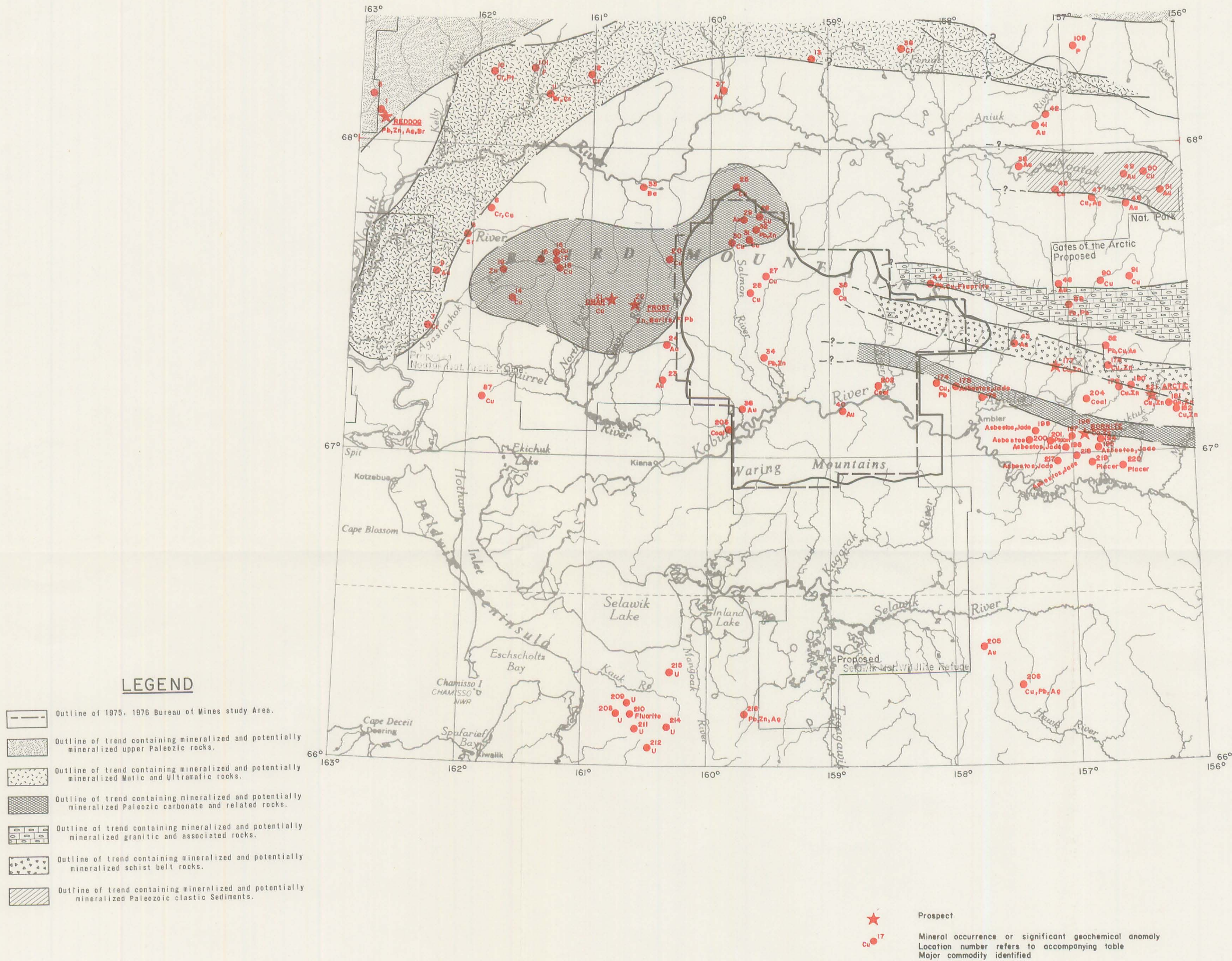
FIGURE 5. - Zones favorable for discovery of additional mineral deposit in the proposed Kobuk Valley National Monument
