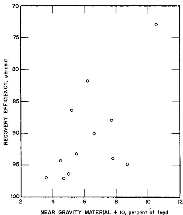
FIGURE 1. - Relation Between Recovery Efficiency and Amount of Near-Gravity Material.
