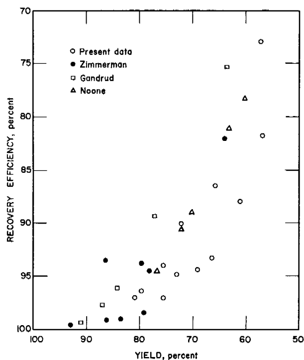
FIGURE 2. - Relation Between Recovery Efficiency and Yield.
