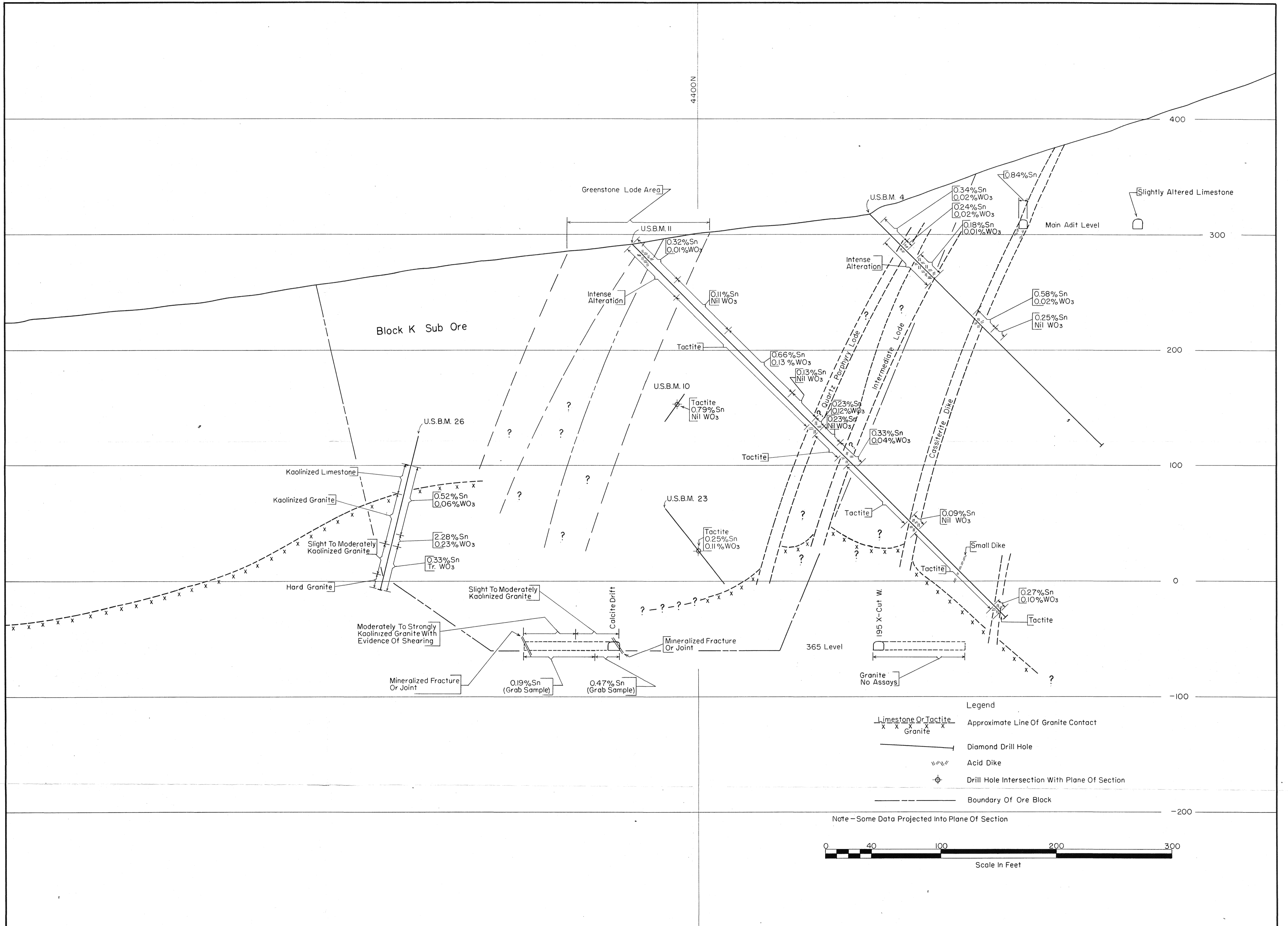
Figure B9 Section CC', Lost River Mine
