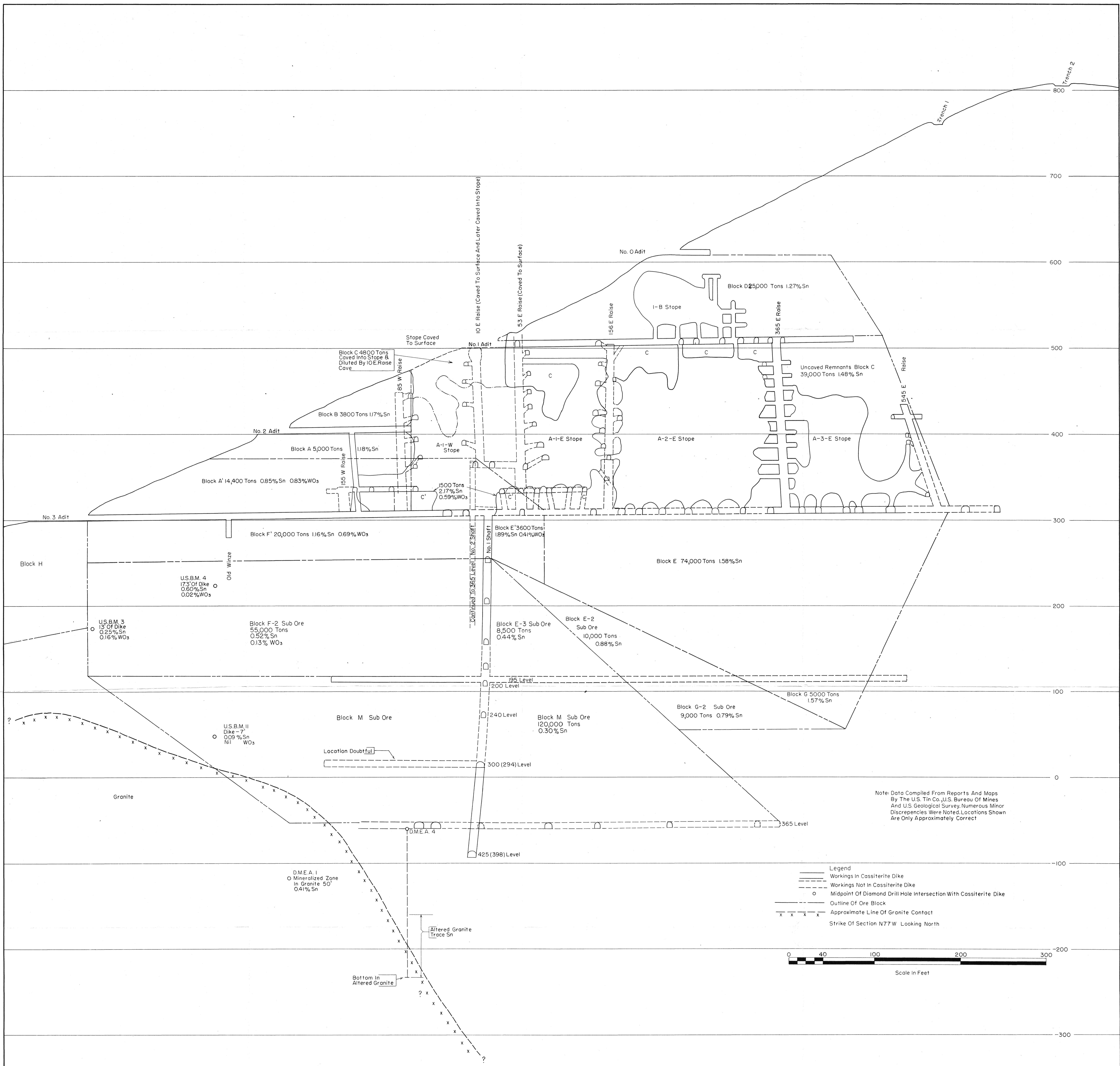
Figure B-II Vertical Longitudinal Section, Cassiterite Dike, Lost River Mine
