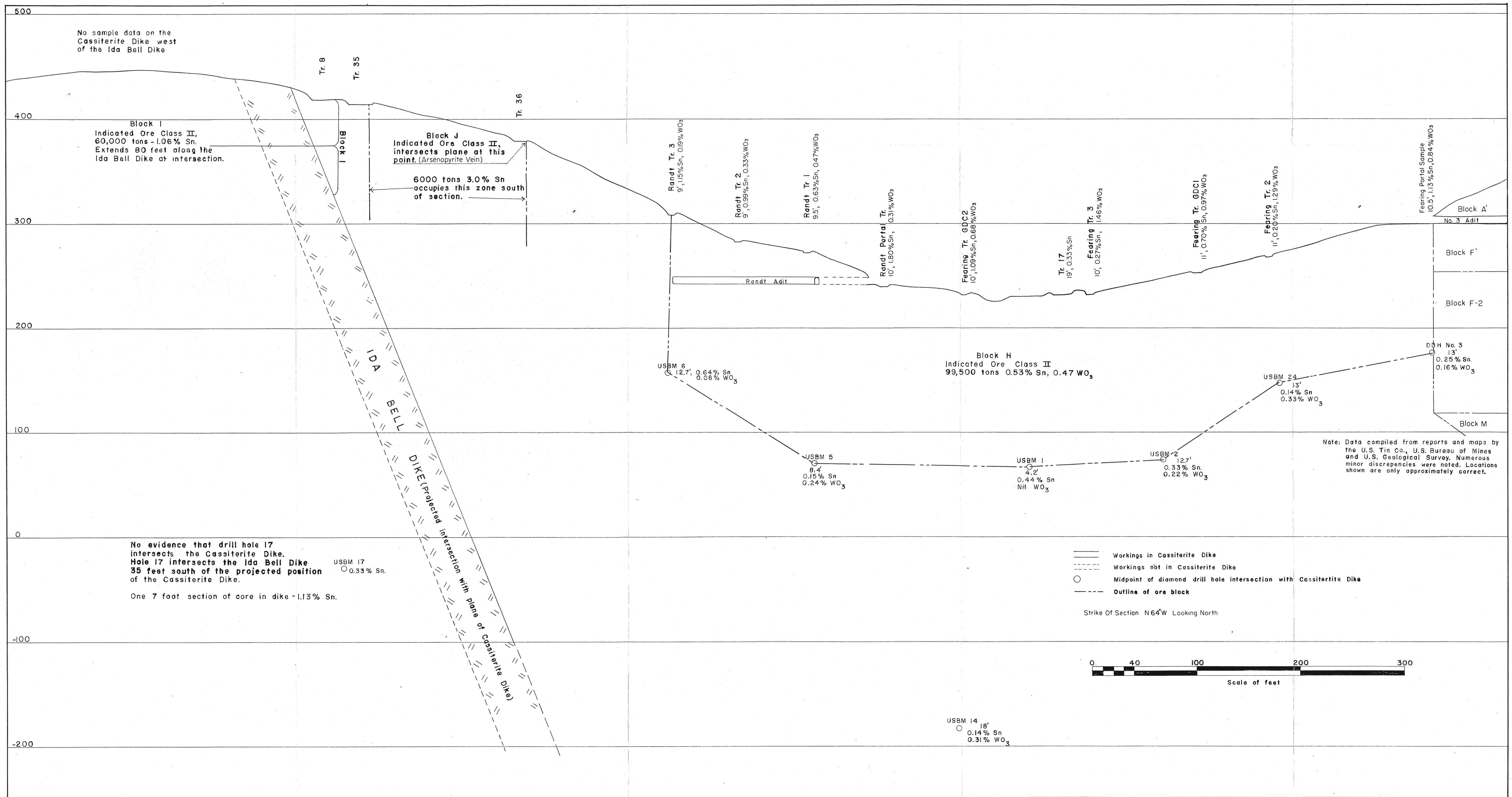
Figure B-12. - Vertical longitudinal section, Cassiterite Dike, Lost River Mine.
