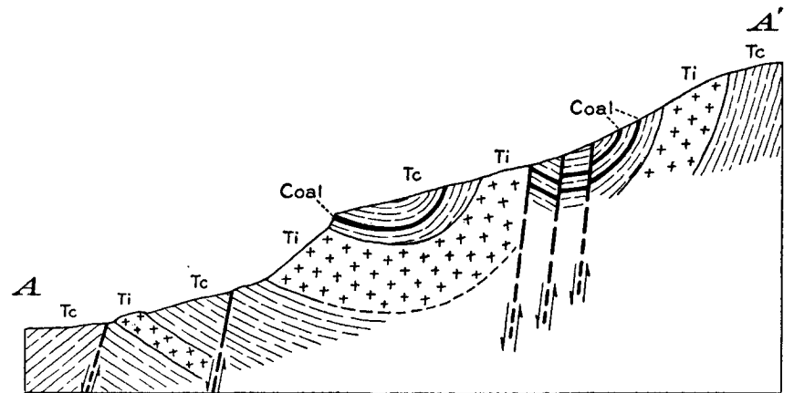
Section along line A-A
