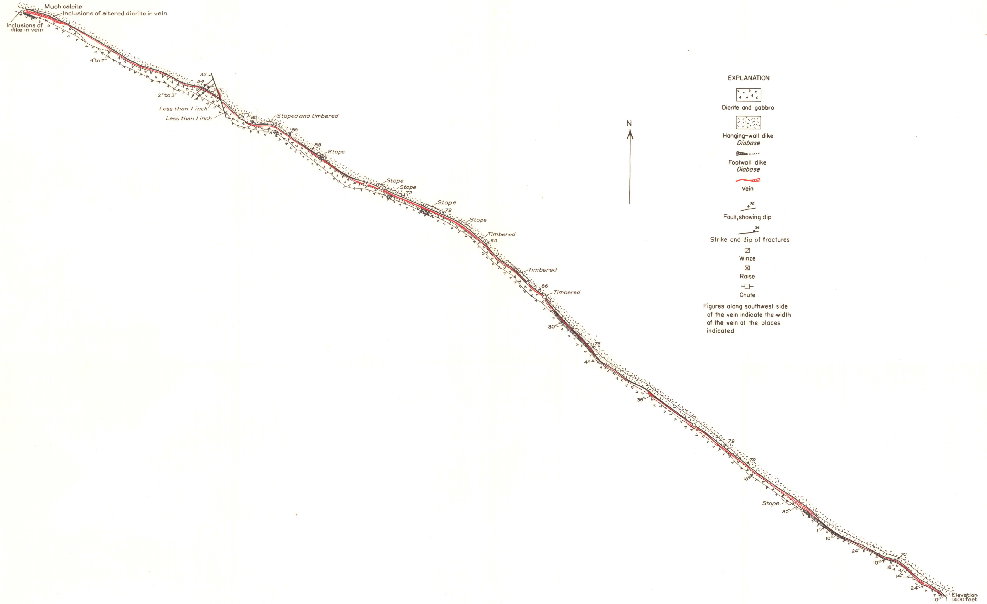
GEOLOGIC MAP OF THE MAIN LEVEL OF THE FLAGSTAFF MINE, PRINCE OF WALES ISLAND, SOUTHEASTERN ALASKA
