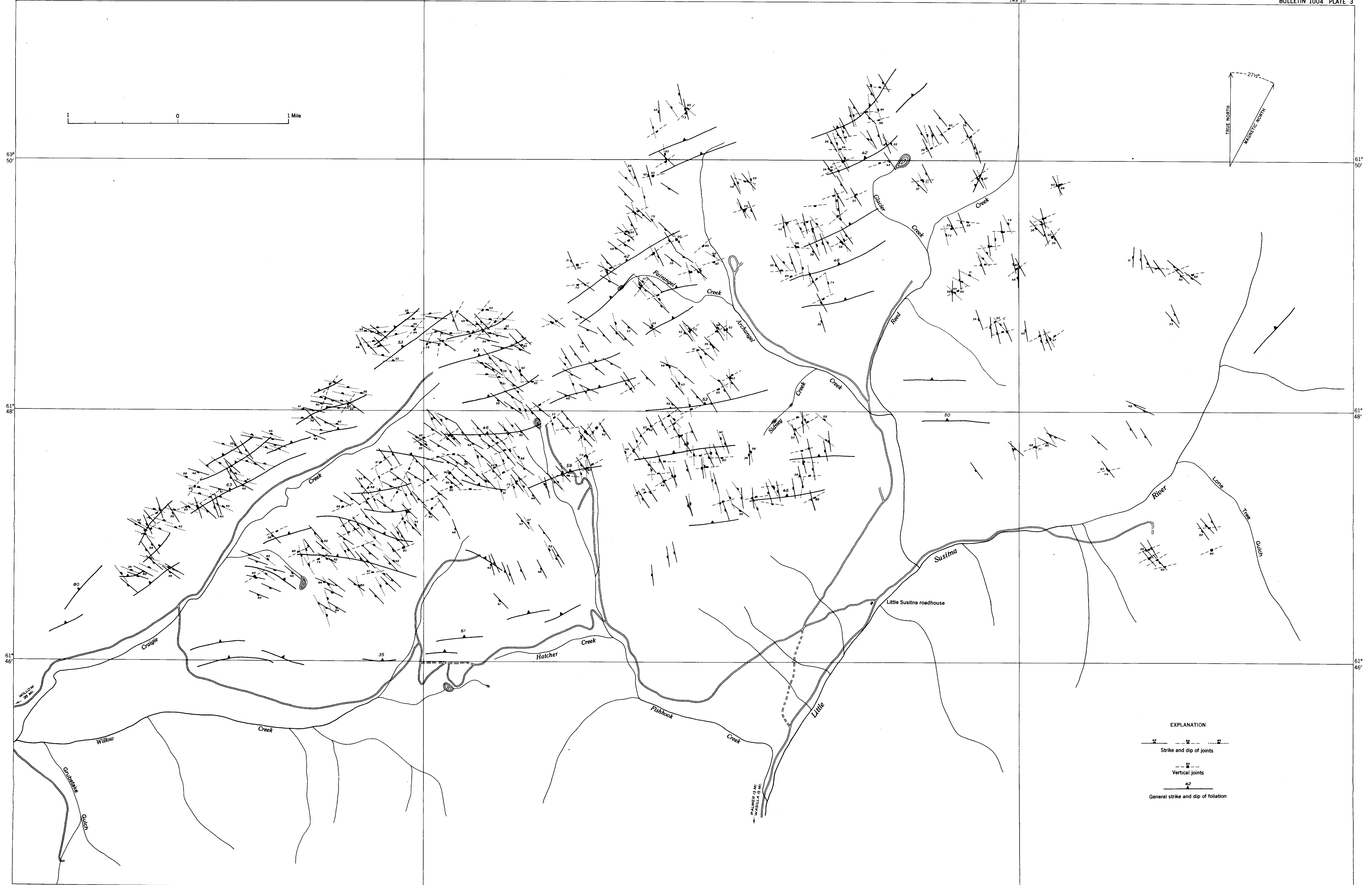
MAP SHOWING JOINT SYSTEM AND GENERAL FOLIATION PATTERN IN QUARTZ DIORITE, WILLOW CREEK MINING DISTRICT, ALASKA
