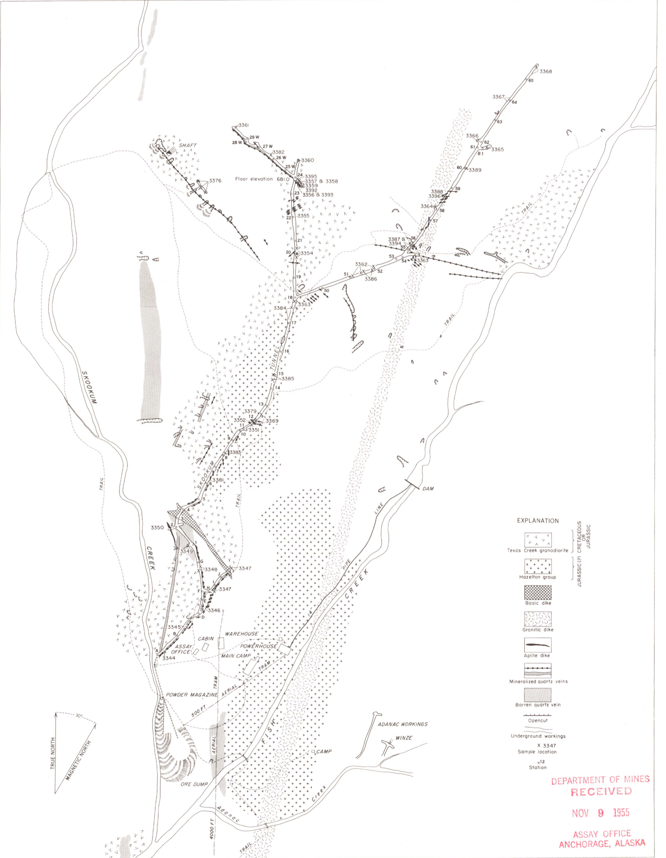
GEOLOGIC SKETCH MAP SHOWING LOCATION OF UNDERGROUND SAMPLES ON PART OF THE MOUNTAIN VIEW PROPERTY, HYDER DISTRICT, ALASKA
