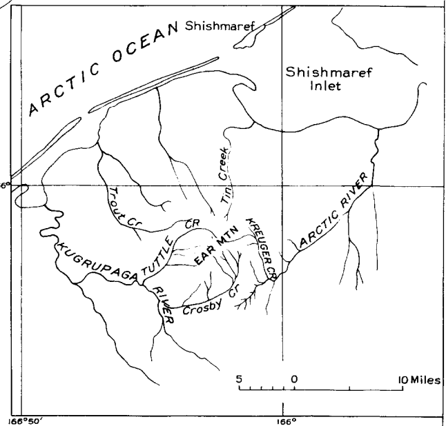
RELATION OF CREEKS TO MAJOR DRAINAGE PATTERN
