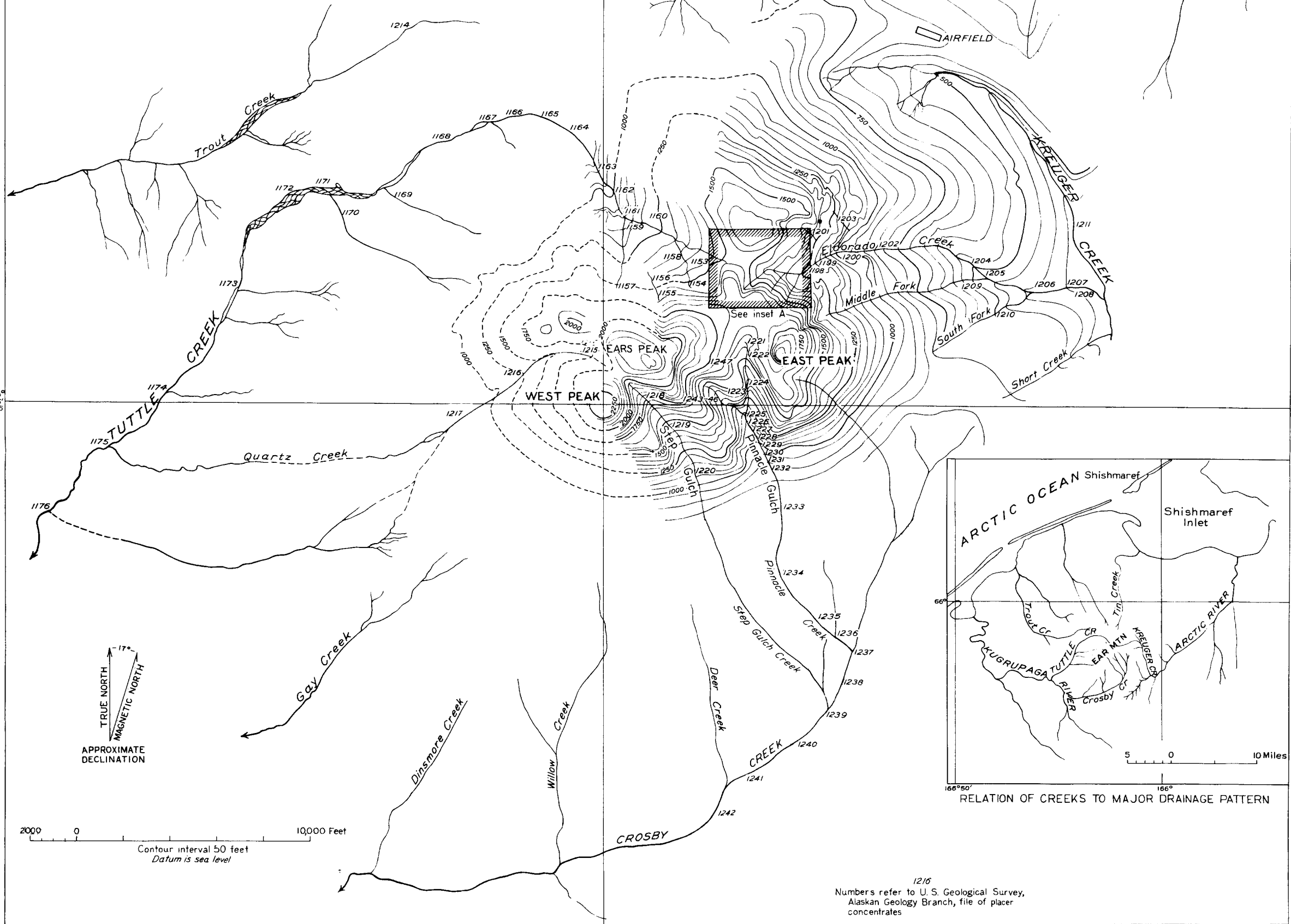
SKETCH MAP OF EAR MOUNTAIN AND VICINITY, SEWARD PENINSULA, ALASKA
