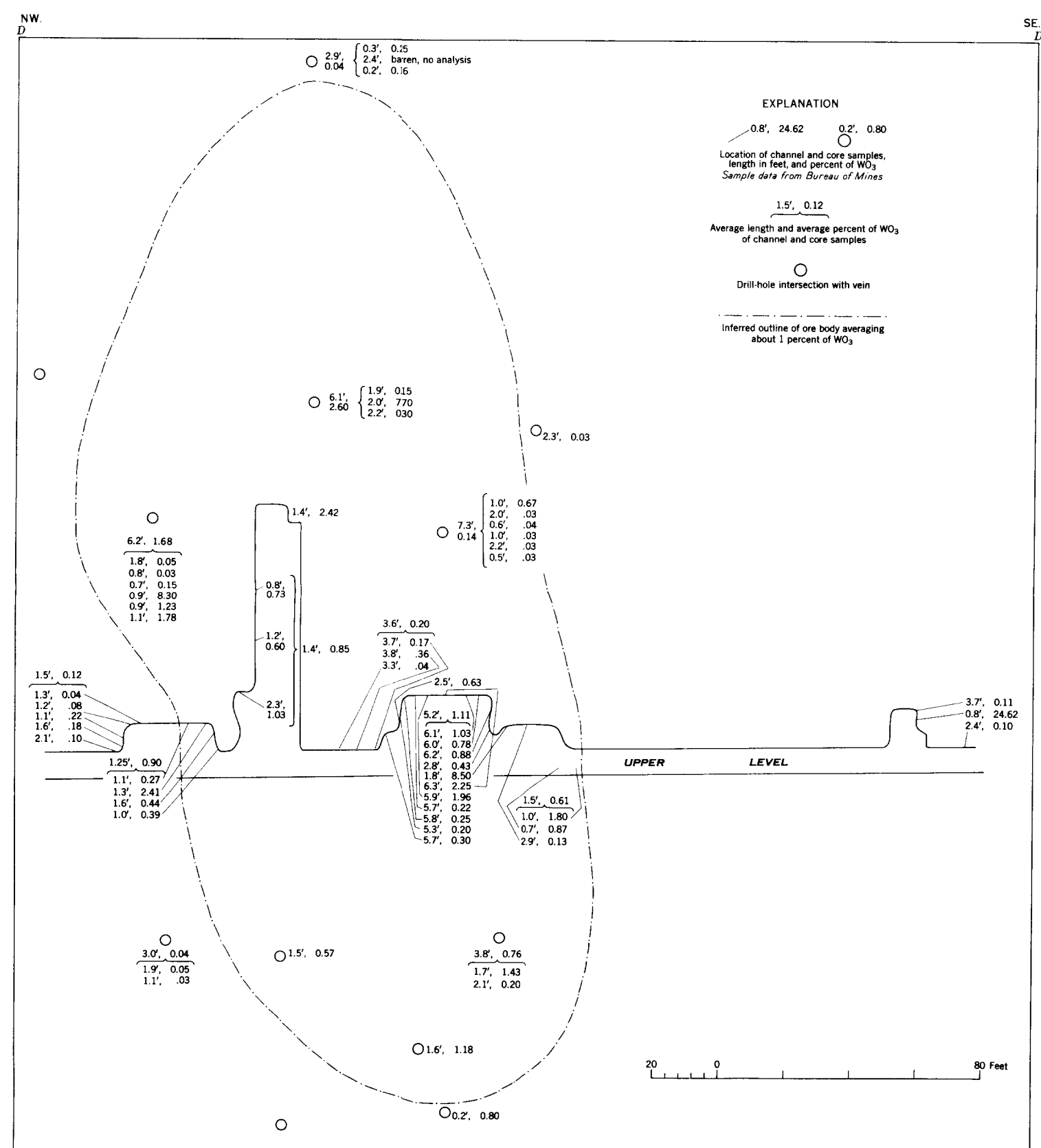
LONGITUDINAL PROJECTION OF MAIN WORKINGS IN LINDBORG SHEAR ZONE, SHOWING DISTRIBUTION OF SCHEELITE, RIVERSIDE MNE (1942), HYDER DISTRICT, ALASKA
