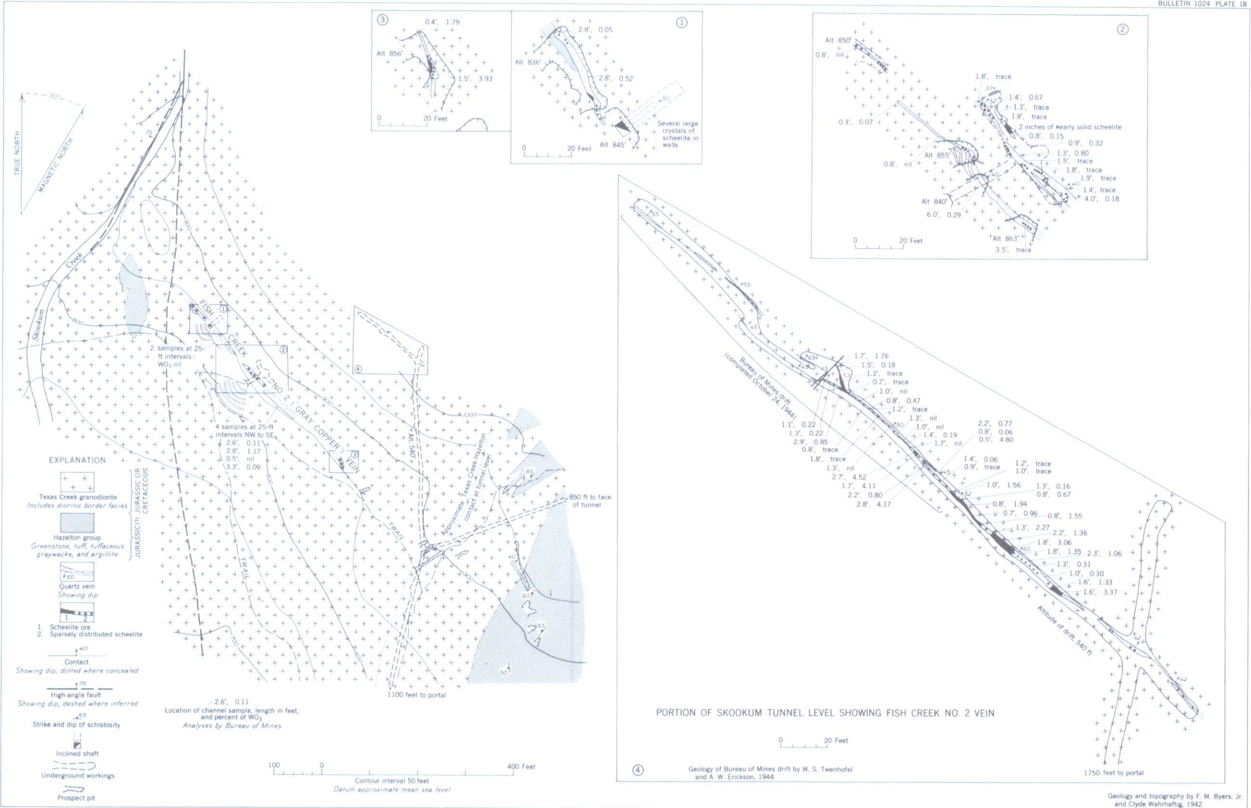
GEOLOGIC MAP SHOWING SCHEELITE DEPOSITS OF THE MOUNTAIN VIEW PROPERTY, HYDER DISTRICT, ALASKA
