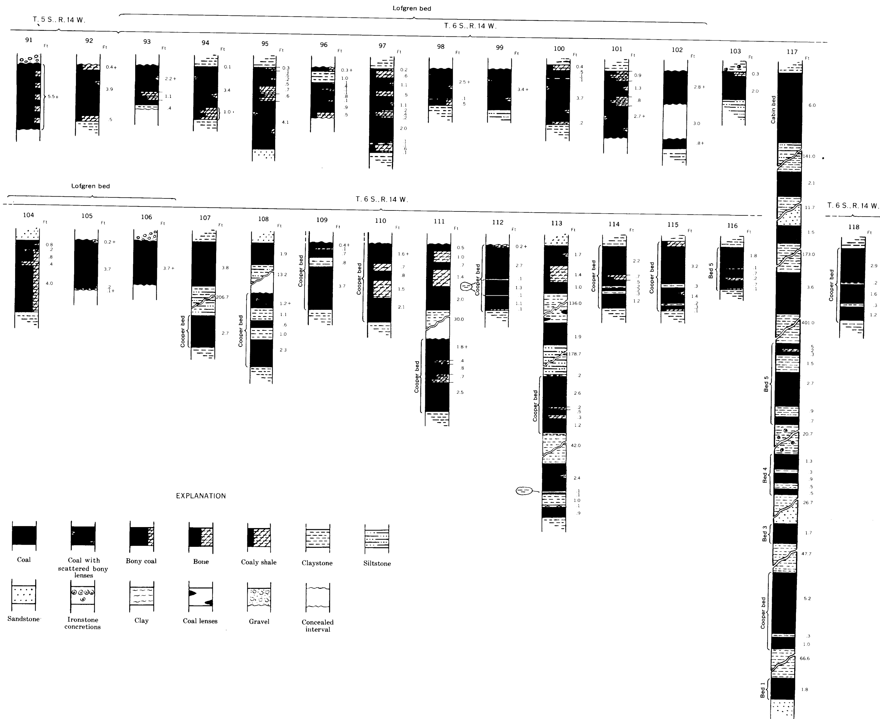
SECTIONS OF COAL BEDS AT LOCALITIES 91 TO 118 IN T. 5 S. AND T. 6 S., R. 14 W. HOMER DISTRICT, ALASKA
