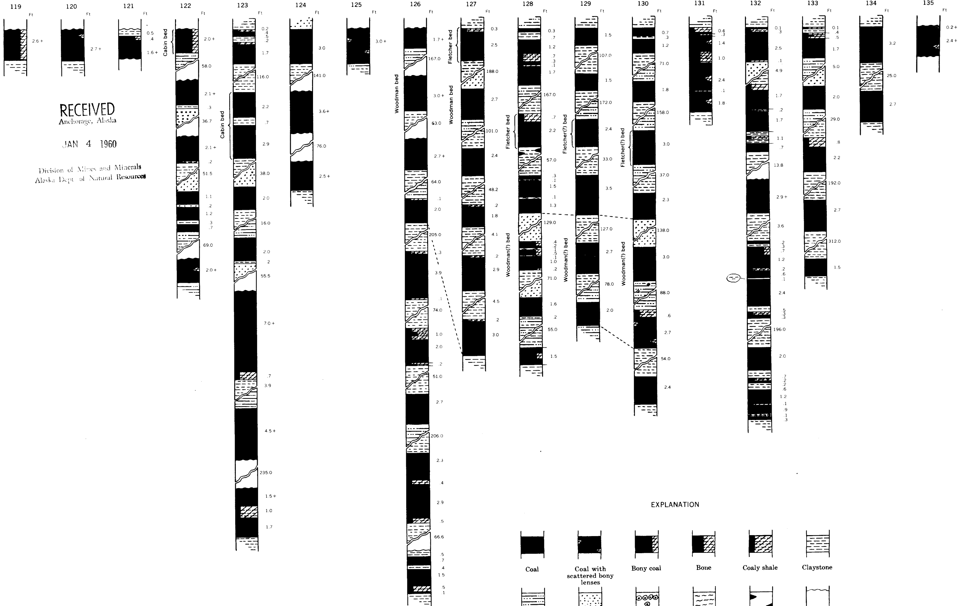
SECTIONS OF COAL BEDS AT LOCALITIES 119 TO 135 IN T. 5 S. AND T. 6 S., R. 12 W. AND R. 13 W., HOMER DISTRICT, ALASKA
