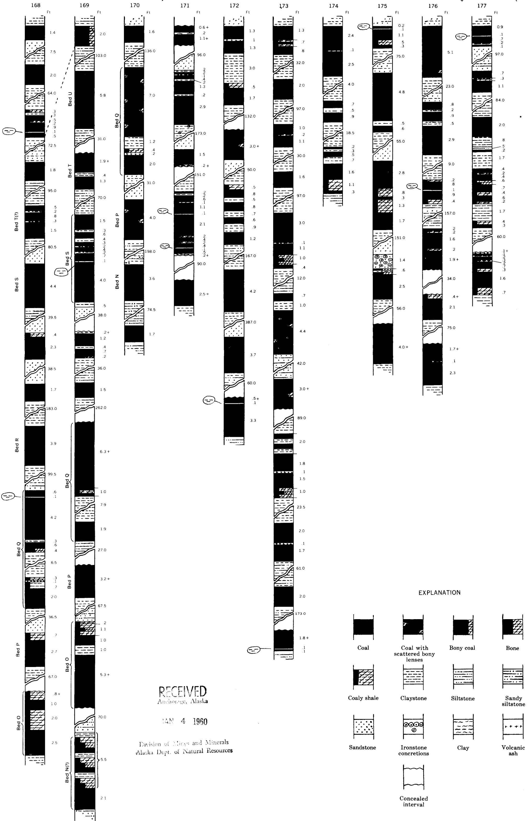
SECTIONS OF COAL BEDS AT LOCALITIES 168 TO 177 NORTH OF THE HEAD OF KACHEMAK BAY, HOMER DISTRICT, ALASKA
